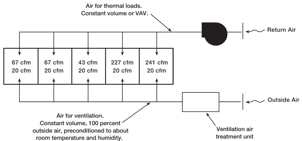
Figure 4-3: De-coupled System
