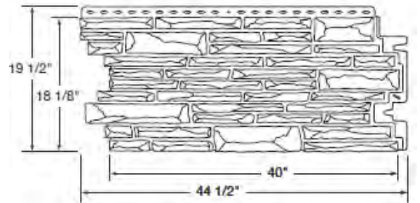
PANEL DIMENSIONS
