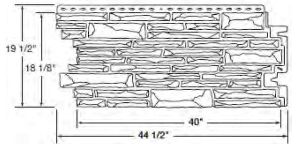
PANEL DIMENSIONS
