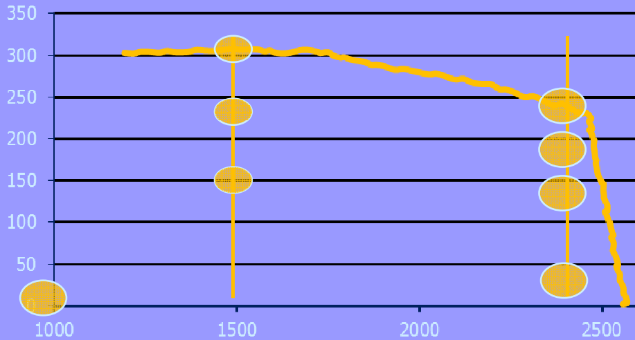
Engine Torque (lb-ft) vs Engine RPM
