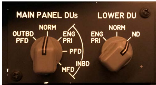
Selecting the Captain's ND to the lower DU
