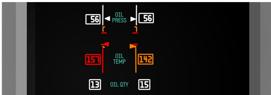
High Oil Temperature Indication (left engine: above redline, right engine: in caution range)
