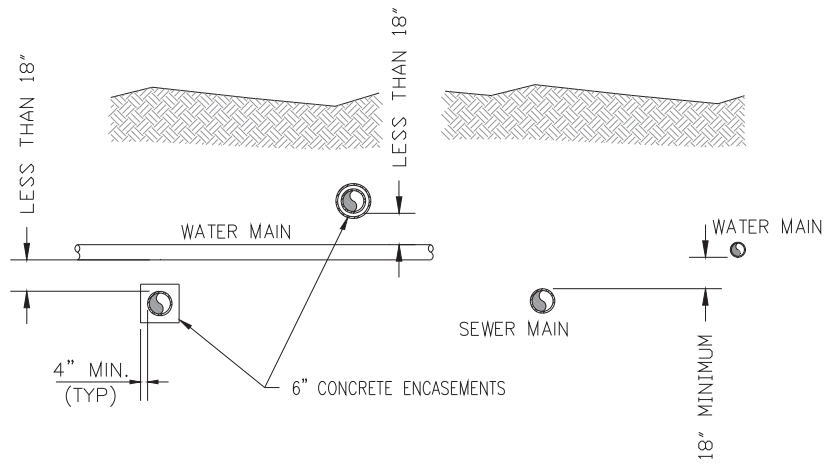
SECTION VIEW
