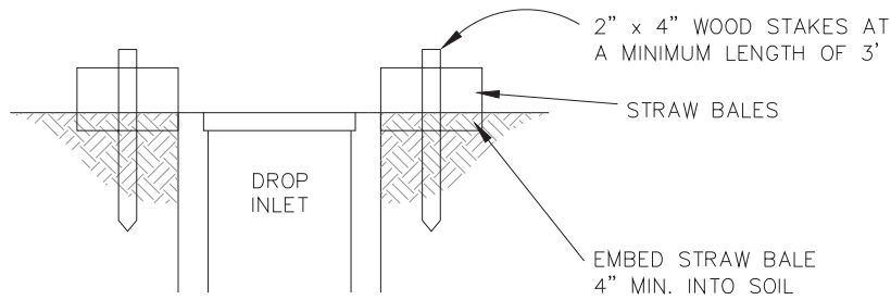
SECTION VIEW
