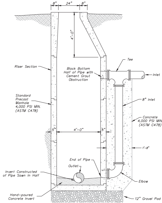
STANDARD SEWER MANHOLE WITH DROP CONNECTION NOT TO SCALE
