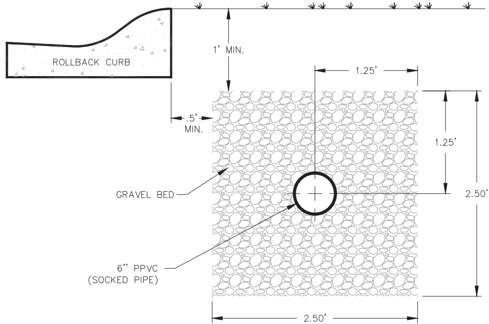
SECTION VIEW
