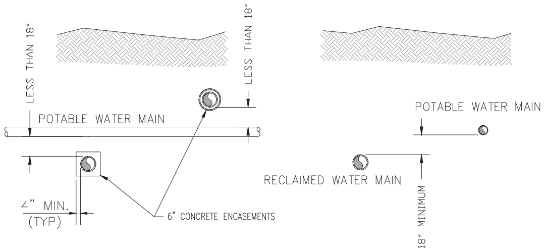
SECTION VIEW
