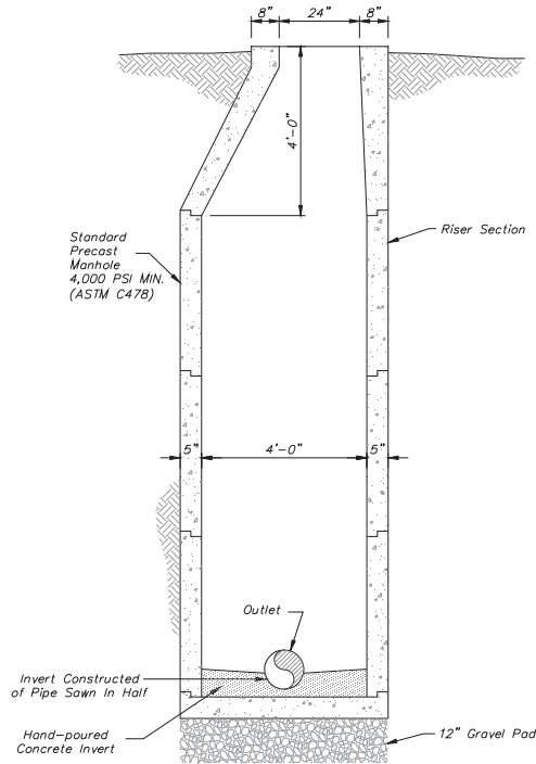
STANDARD SEWER MANHOLE NOT TO SCALE
