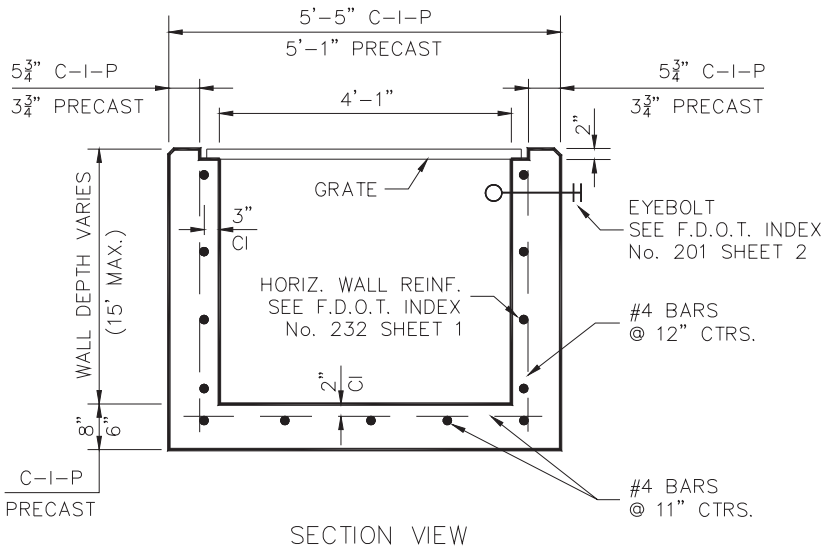
TYPE "D" CATCH BASIN DETAIL (F.D.O.T. INDEX No. 232)
