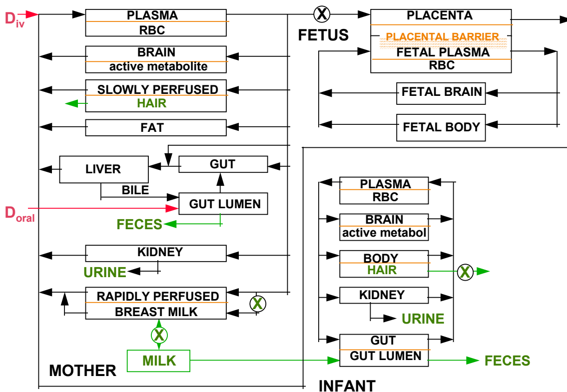
Figure 2-1. A diagram of the conceptual framework for the physiologically based pharmacokinetic (PB/PK) model of gestational/lactational transfer of a potential developmental toxicant from the exposed mother to her nursing infant
