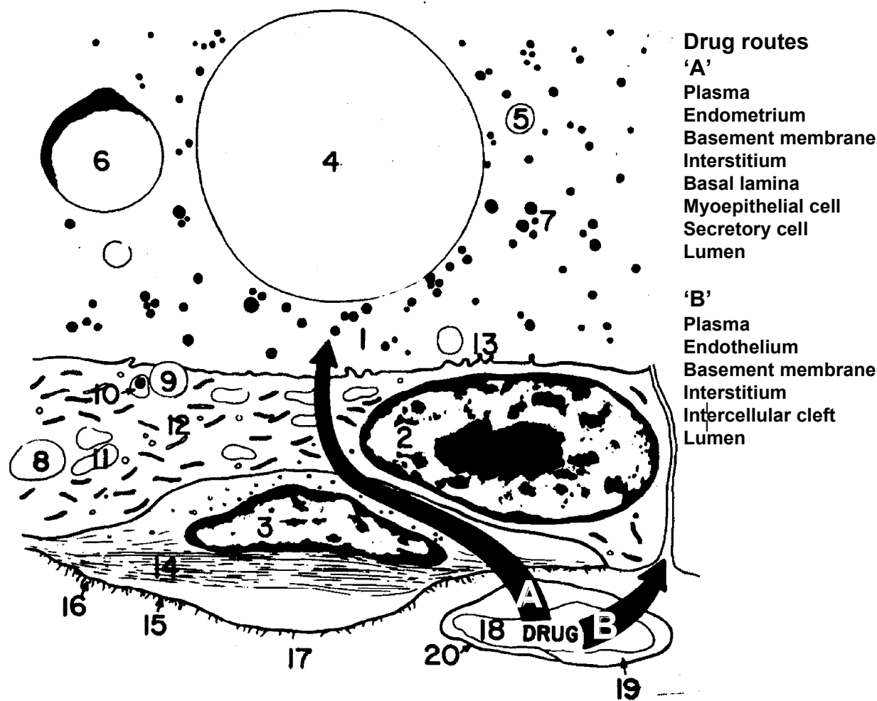
Figure 4-1. A scheme of a lactational transfer of a chemical from maternal blood (redrawn with permission from Wilson et al., 1980)
