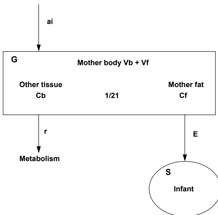
Figure 4-7. Schematic diagram of the linear, one-compartment open pharmacokinetic system described mathematically by Hoover et al. (1991)
