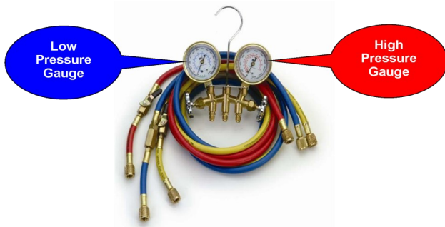
Figure 2. Manifold and Hose Set
