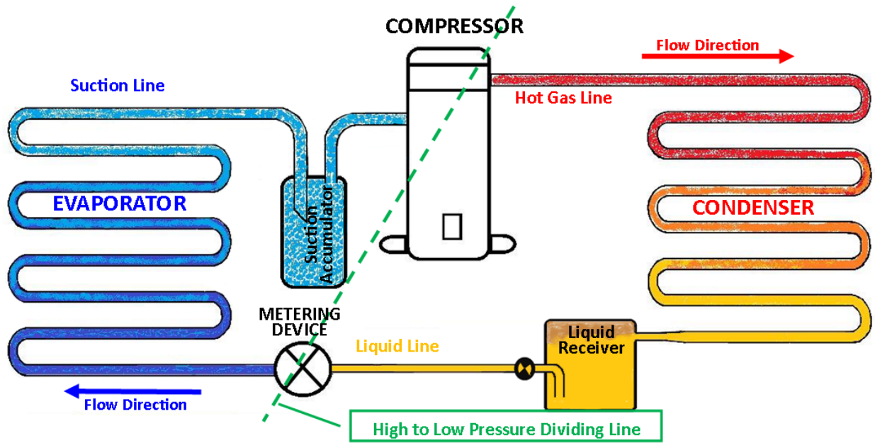
Figure 1. Basic Vapor/Compression Refrigeration Cycle
