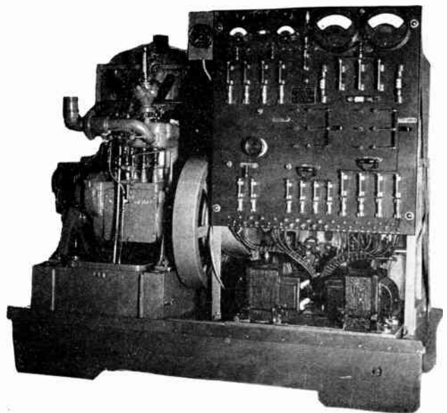
Figure 2. 5-kw ac-dc "portable" unit, 1920—Control panel side
