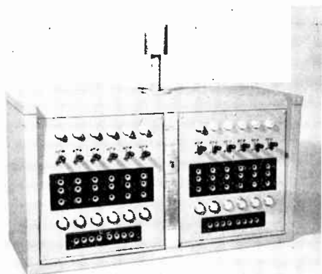
Figure 8. Network Dispatcher Turret 6624-A
