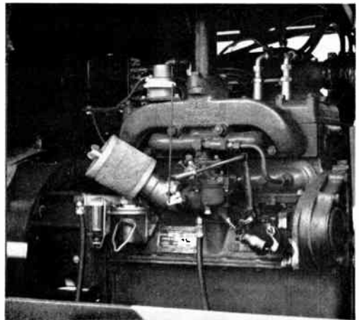
Figure 10. Engine—Carburetor side
