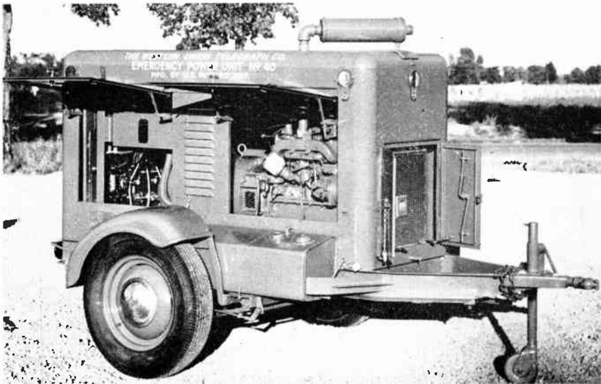
Figure 1. Modern trailer-mounted portable power unit
