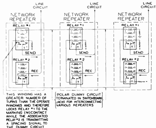
Figure 1. Theory of dummy circuit used on existing repeaters to interconnect a number of line circuits into one half-duplex network
