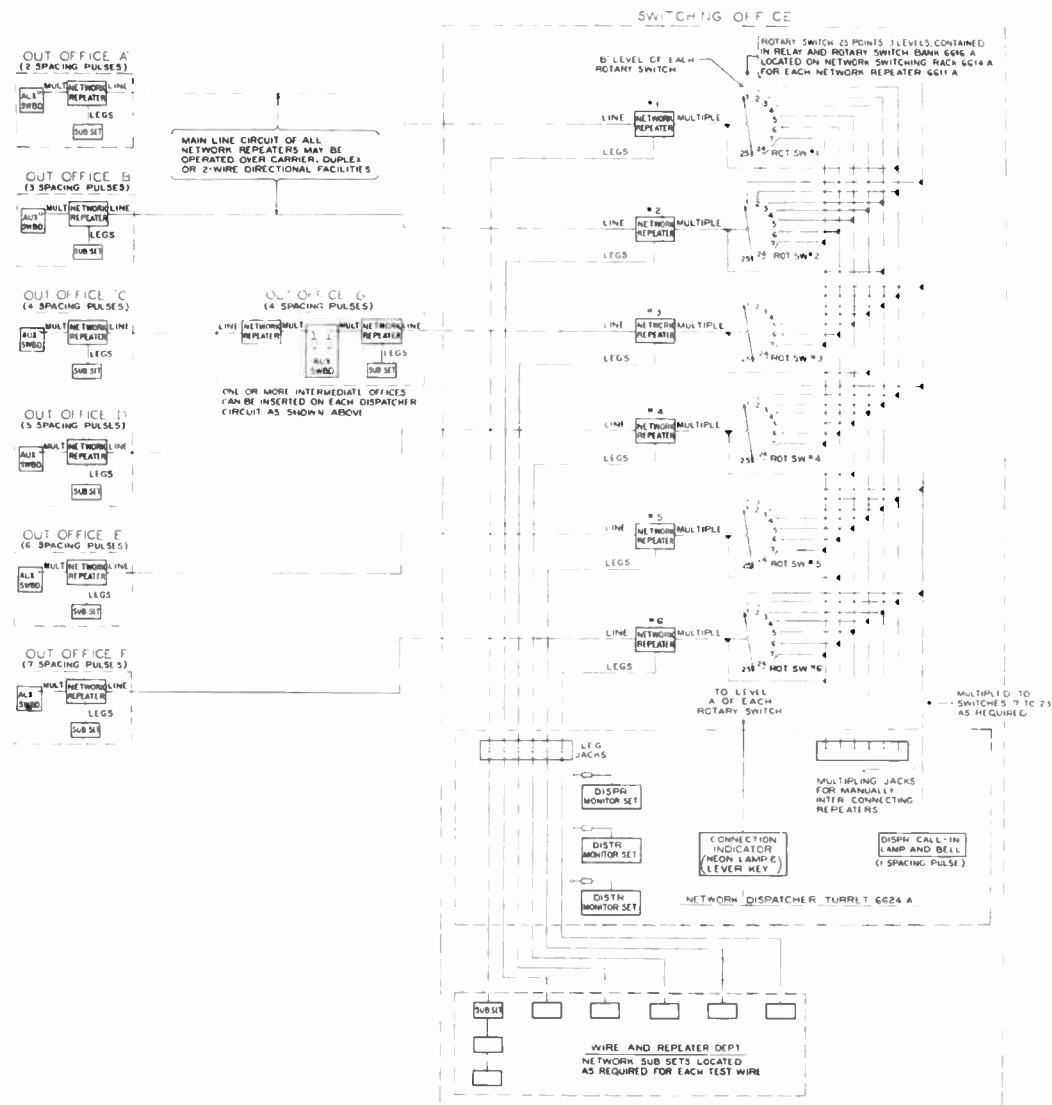
Figure 4. Theory of Network Switching System, Plan 101-A
