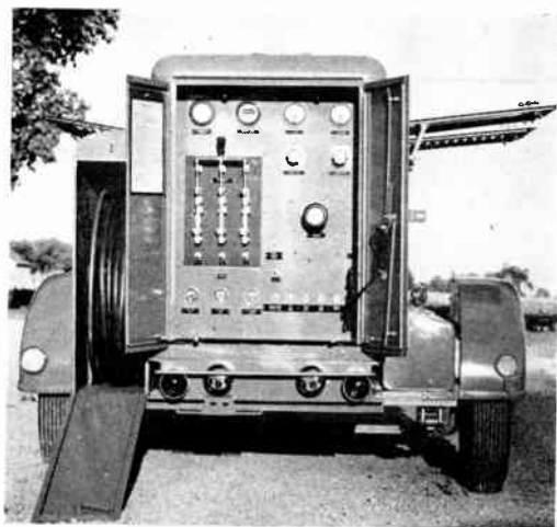
Figure 7. Control panel and cable reels
