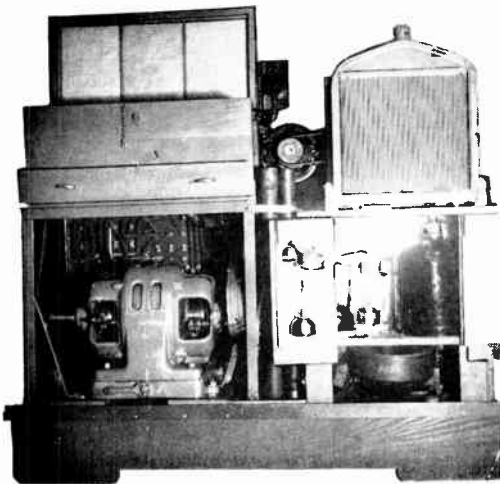
Figure 3. 1920 "portable" unit—Generator side
