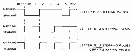
Figure 7. Method of transmitting selection code by using teleprinter keyboard character combinations
