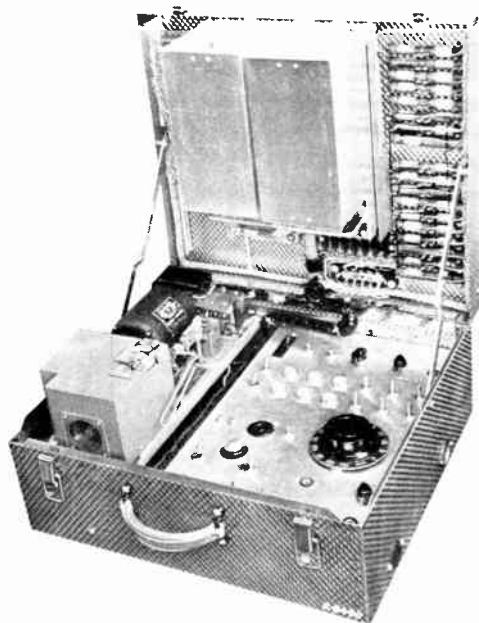
Portable Test Set 6030-B and Distributor-Transmitter 5032-A
