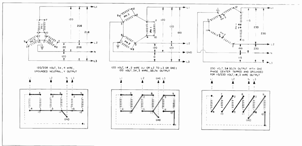
Figure 11. Theoretical alternator coil connections and arrangement of straps on terminal panel
