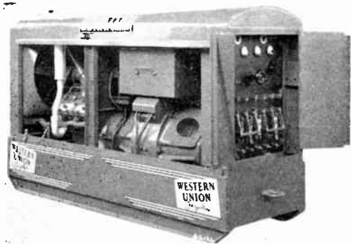
Figure 4. 25-kw ac-dc portable unit—1938
