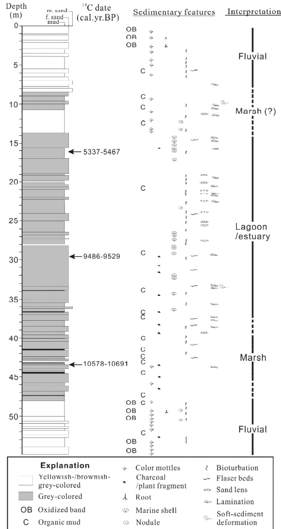
Fig. 3. Upper 55 m sequence of Lu-tso core. For location see Fig. 1. Ground surface is 14.6 m above sea level. Sediments dated 9486 - 9529 cal.yr.BP ( 1\sigma range) are interpreted as deposited -3 to 0 m of the coeval mean sea level, as they are rich in organic materials and contain marine shells. Sediments dated 10578-10691 cal.yr.BP are interpreted as deposited 0 to 3 m of the sea level, as they are associated with weakly-oxidized strata and are close in sequence to marine-shell-bearing strata. These two dates are used in testing eustatic sea level (Table 1). Date 5337-5467 cal.yr.BP is derived from marine-shell-bearing strata. However, as the sediments do not include abundant organic materials, their deposition position is not well constrained (merely < 0 m of the sea level).
