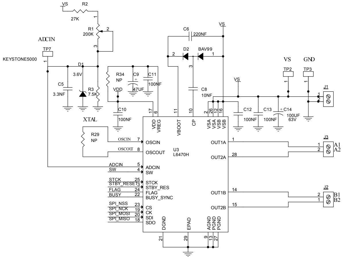
Figure 4. Schematic (motor driver part)
