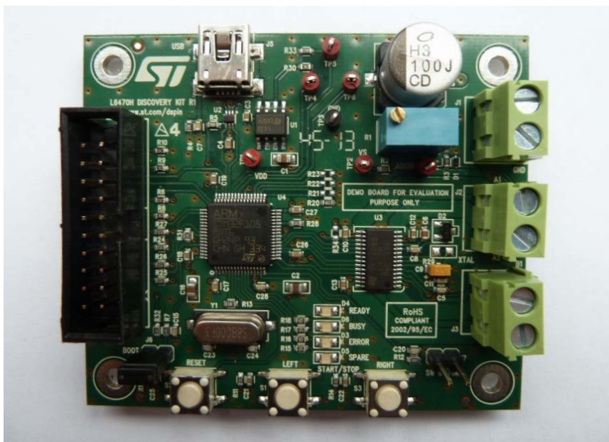
Figure 1. EVAL6470H-DISC board
