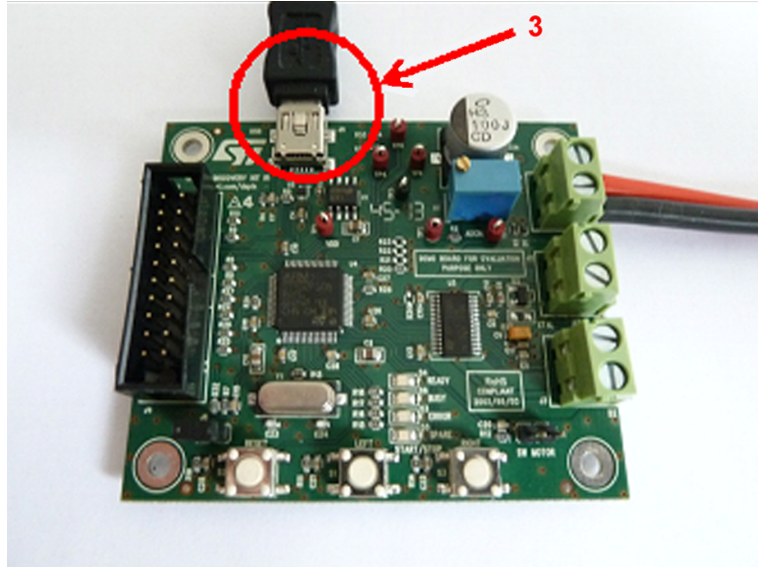
Figure 20. Starting board (USB connection)
