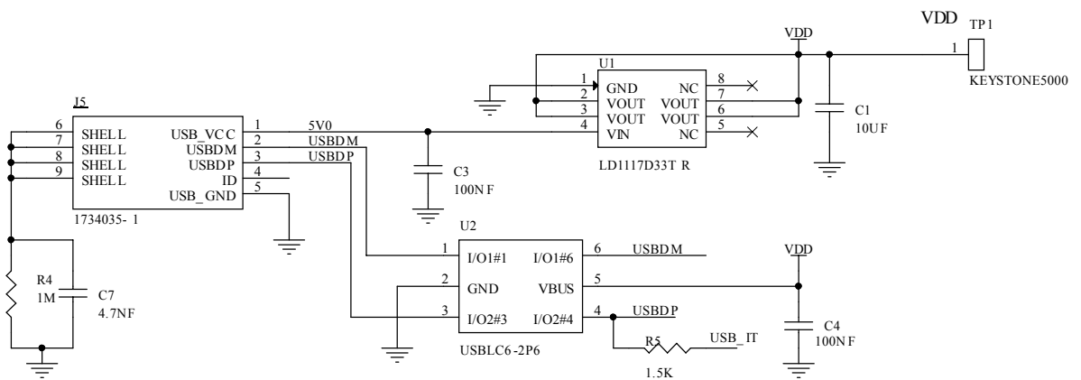
Figure 6. Microcontroller supply section
