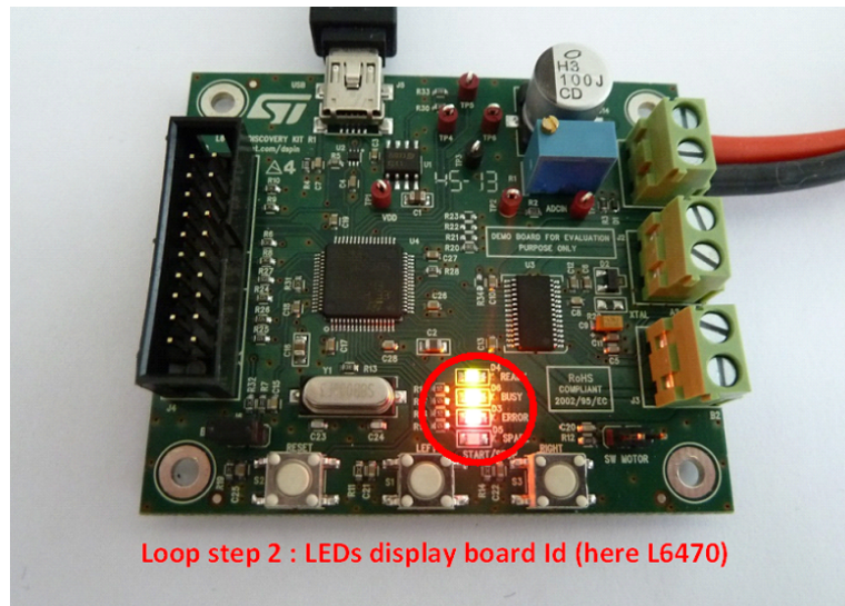
Figure 23. Starting board (display board ID)
