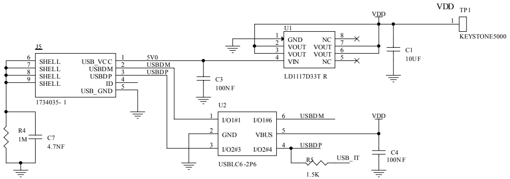
Figure 2. Schematic (microcontroller supply part)
