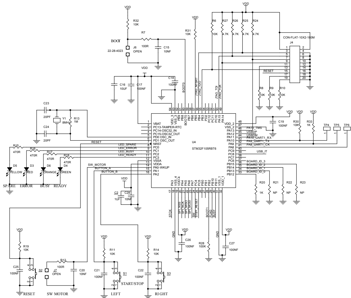
Figure 3. Schematic (microcontroller part)
