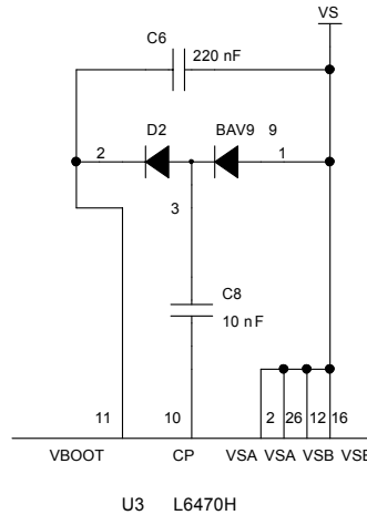
Figure 8. Charge pump circuitry
