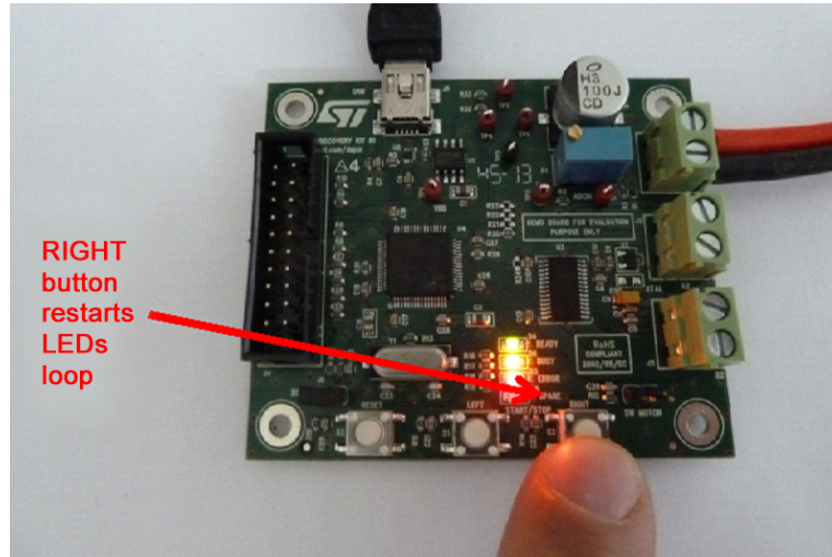
Figure 25. Starting board (action RIGHT key)
