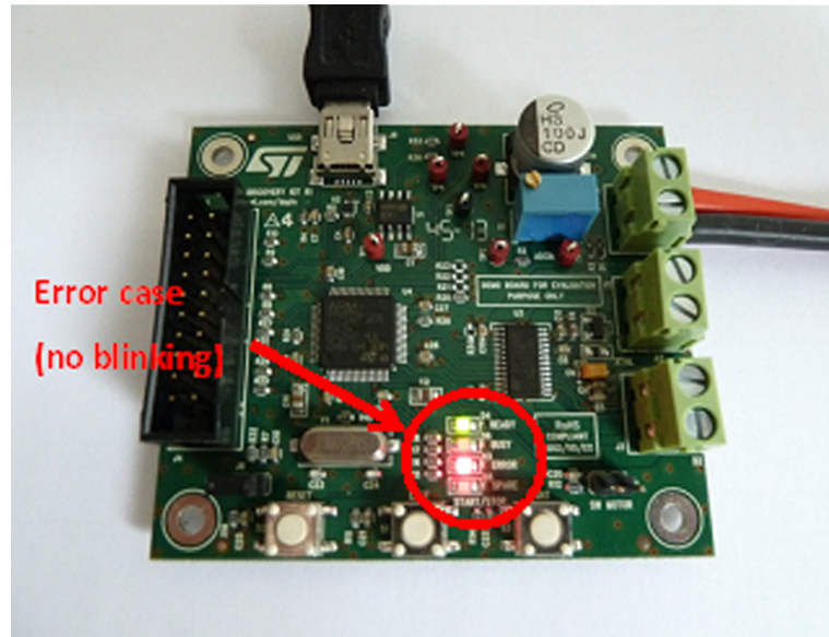
Figure 21. Starting board (error case)
