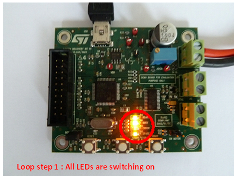
Figure 22. Starting board (board OK)
