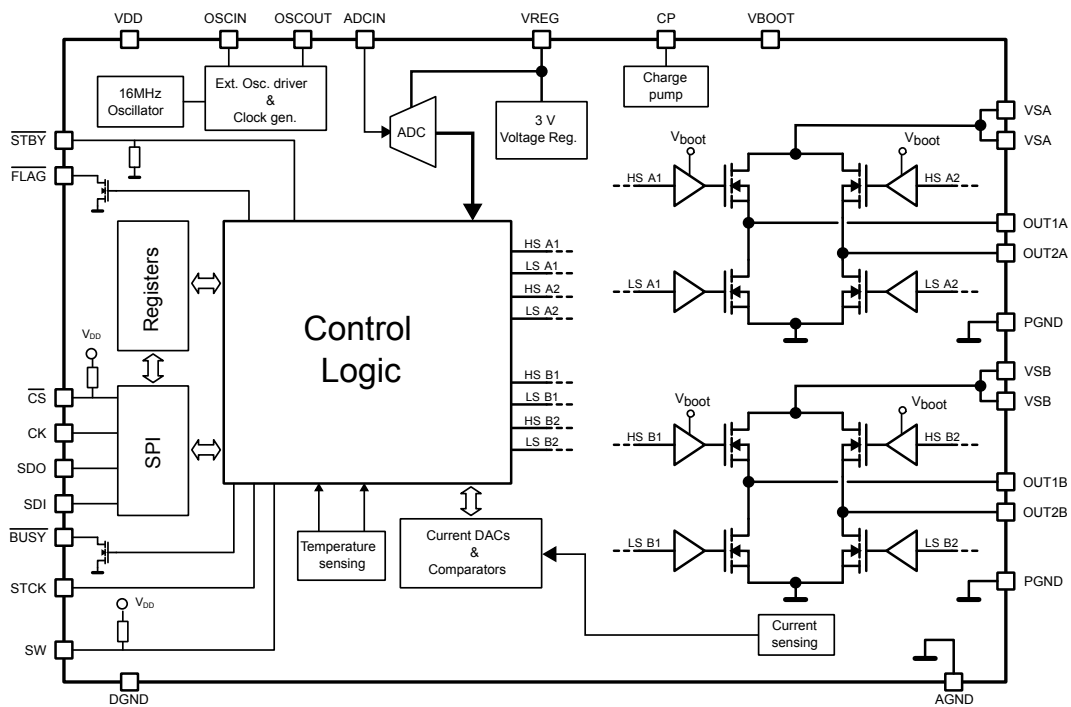
Figure 7. L6470 block diagram
