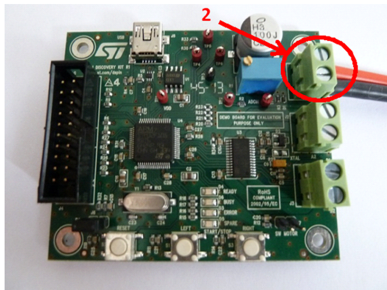
Figure 19. Starting board (motor power supply)
