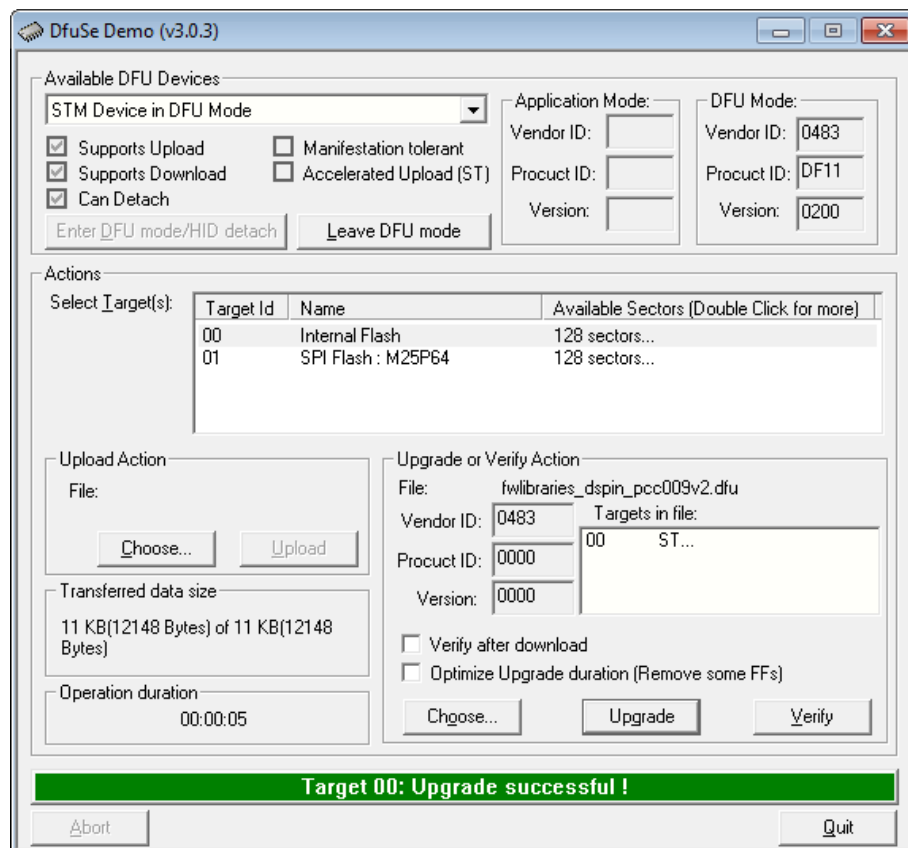
Figure 17. DFU file (download OK)
