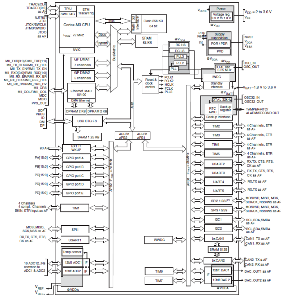
Figure 9. STM32F105xx and STM32F107xx block diagram
