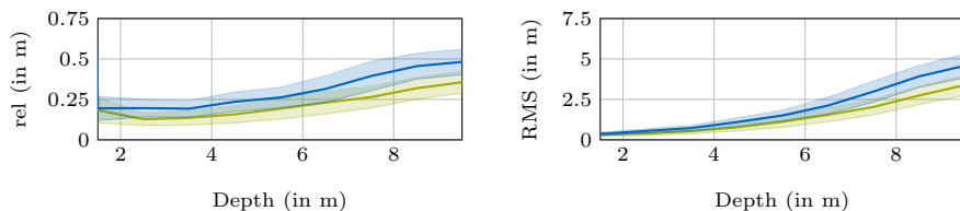
Fig. 5: Distance-related global errors (left: relative error and right: RMS) for NYU-v2 (mean: —, \pm 0.5 std: ■) and iBims-1 (mean: —, \pm 0.5 std: ■) using the method of Li et al. [19]
