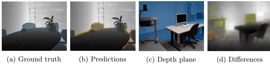
Fig. 7: Visual results after applying DBE (a+b) and DDE (c+d) on iBims-1: (a) ground truth edge (—). (b) Edge predictions using the methods of Li et al. [19] (—) and Laina et al. [15] (—). (c) Ground truth depth plane at d = 3 m separating foreground from background (■). (d) Differences between ground truth and predicted depths using the method of Li et al. [19]. Color coded are depth values that are either estimated too short (■) or too far (■)
