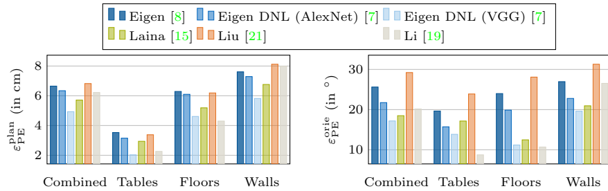
Fig. 6: Results for the planarity metrics \varepsilon_{PE}^{plan} (left) and \varepsilon_{PE}^{orie} (right) on iBims-1
