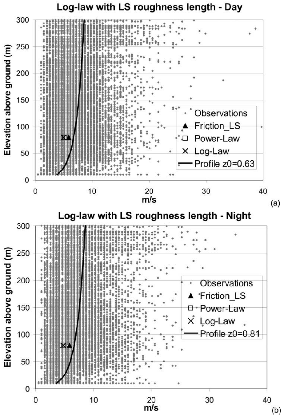
Figure 10. Wind speed observed worldwide in the lowest 300 m, calculated V80 obtained with: z_0^{\text{LS}} (triangle), z_0 = 0.01 (cross), \alpha = 1/7 (square), and profile obtained (a) with the global average z_0^{\text{LS}} = 0.63 (solid line) during the day and (b) with z_0^{\text{LS}} = 0.81 at night.
