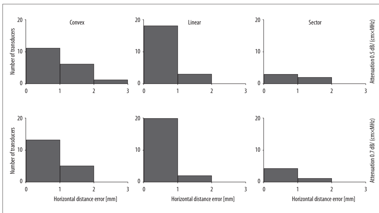
Figure 4. Difference between nominal and measured distance in the horizontal direction.
