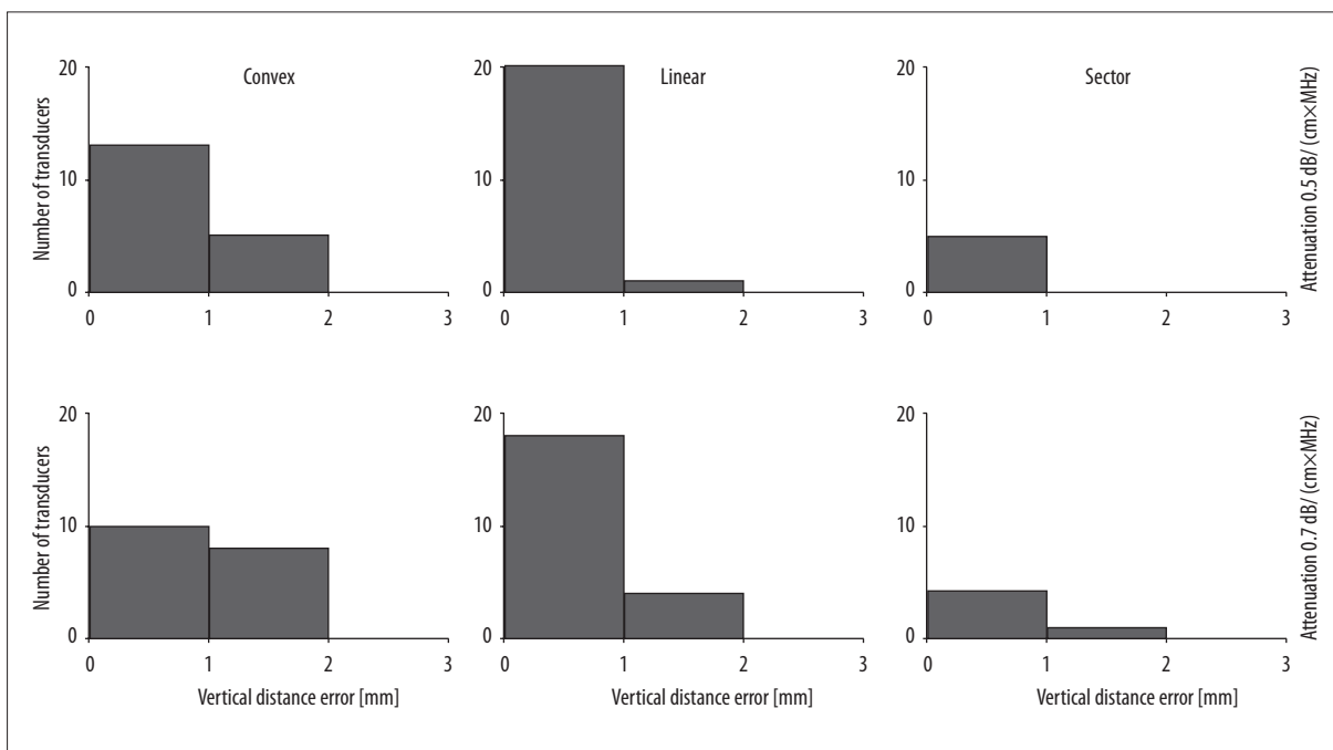
Figure 5. Difference between nominal and measured distance in the vertical direction.
