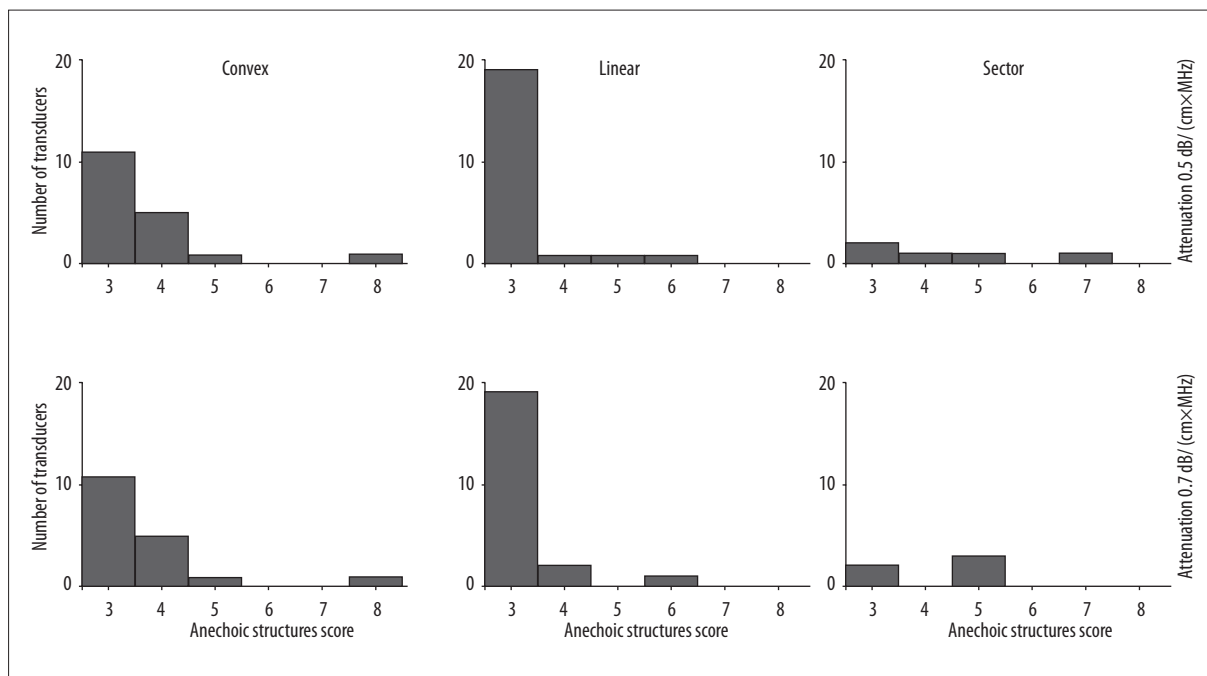
Figure 6. Visibility of anechoic structures. A score of 3 points means no distortions, a higher score represents suboptimal image quality.
