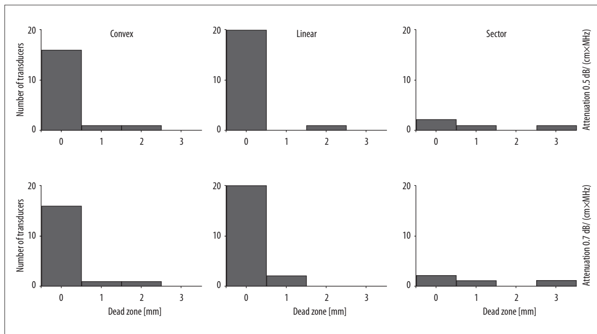
Figure 3. Results of the dead zone test (zero is the best result).
