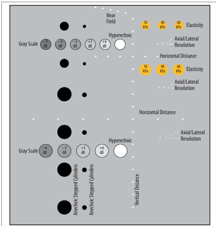
Figure 1. Scheme of the phantom used for evaluation of ultrasound scanners (source: [20]). During measurements, the transducer is in contact with the top surface of the phantom.
