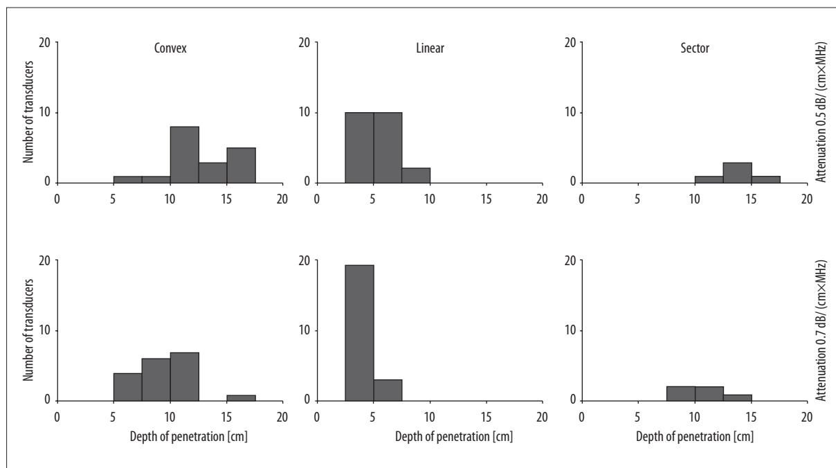
Figure 2. Results of the depth of penetration test.
