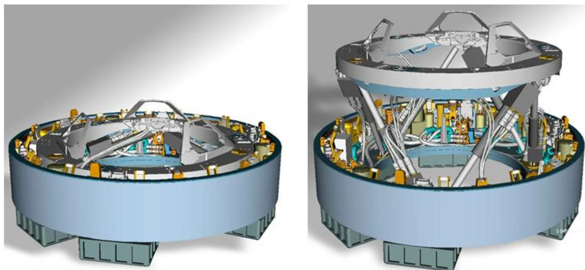
Figure 1 The IBDM equipped with the first generation latching system
