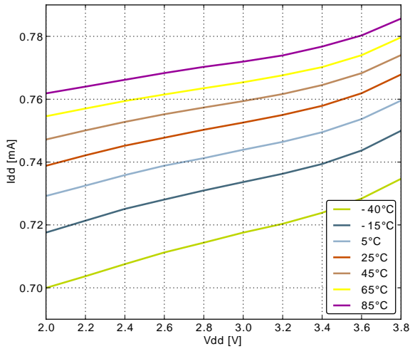
Figure 3.6. EM1 Current consumption with all peripheral clocks disabled and HFRCO running at 6.6MHz
