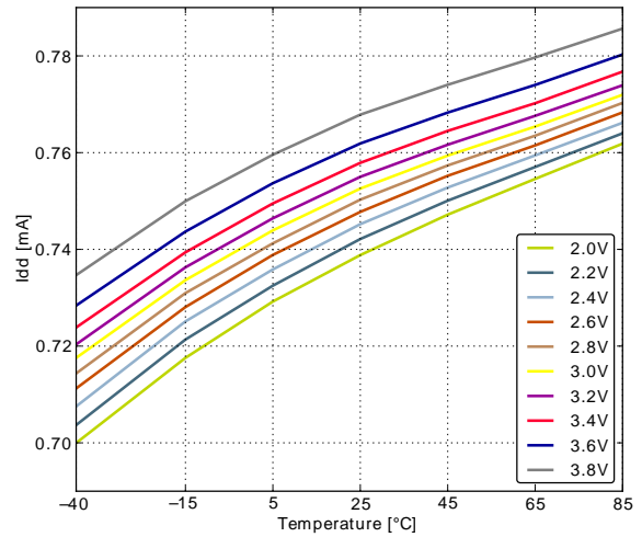
Figure 3.6. EM1 Current consumption with all peripheral clocks disabled and HFRCO running at 6.6MHz
