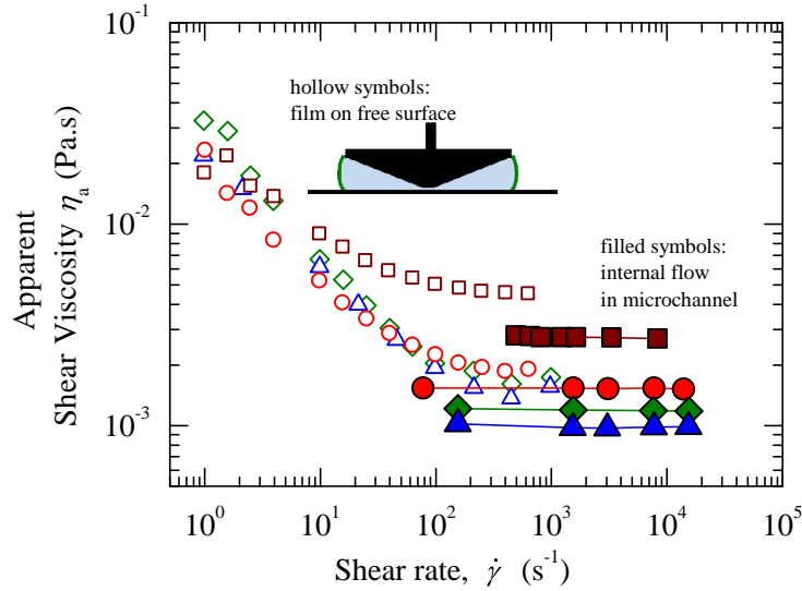
Fig. 12 Surface-active components in solution, such as the protein bovine serum albumin (BSA) shown here, may form a film at a free interface. Such films can show apparent yield stress and shear-thinning of the apparent bulk viscosity when tested with cone plate (hollow symbols). However, this is an interfacial rheological property and not a true bulk property as shown by the internal channel-flow measurements (filled symbols). BSA at bulk concentrations of 10–200 mg/mL, triangles–squares. (Data originally reported by Sharma et al. [51].)
