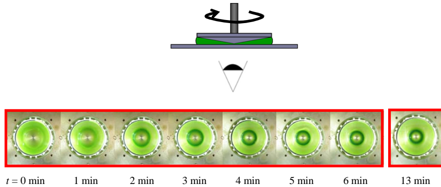
Fig. 16 Visualization can be used to check for nonhomogeneous conditions due to rheotaxis, particle settling, and secondary flow. Here, shear flow of a microalgae suspension is viewed from below through a transparent bottom plate, showing that a non-homogeneous distribution develops over time. (Previously unpublished work of authors RHE and LMC.)
