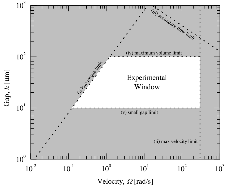
Fig. 15 Experimental window for small volume aqueous solutions, using Eqs. 34–38 to draw the boundaries. Representative values used are T_{\min} = 5 \text{ nN}\cdot\text{m} , \Omega_{\max} = 300 \text{ rad/s} , \text{Re}_{\max} = 4 , \eta = 1 \text{ mPa}\cdot\text{s} , \rho = 1000 \text{ kg/m}^3 , plate diameter D = 8 \text{ mm} , V_{\max} = \mu L , and minimum gap h_{\min} = 10 \text{ }\mu\text{m} .
