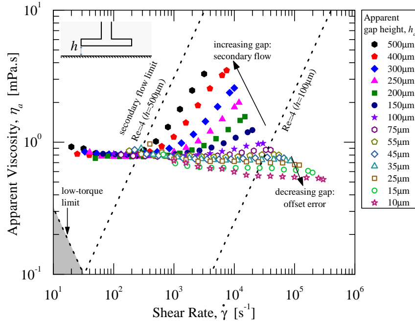
Fig. 14 Small gap/volume measurements of water with plate geometry, D = 20 mm. Gap offset artifacts are seen for apparent gap heights h_a < 50 \mu\text{m} . Inertial secondary flow artifacts appear for sufficiently large Reynolds number, i.e. at larger gaps and high shear rate (Section 3.3). (Previously unpublished work of authors RHE and MTJ.)
