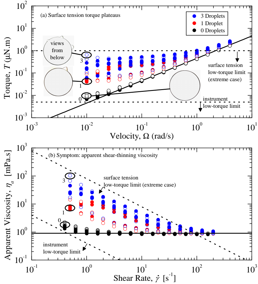
Fig. 10 Surface tension can generate torque in steady shear (a), which could be mistaken as shear thinning (b), as shown here with water at room temperature. The effect grows with slight overfilling that increases contact line rotational asymmetry, here with 1 or 3 small extra droplets of water at the boundary, yet the effect can be present even with best practices (“0 droplets”) where residual torque plateaus appear above the instrument low-torque limit. Views from below in (a) indicate droplet contact lines around the D = 40 mm plate, as viewed through a glass bottom plate. Low-torque limits for \eta_{\min} drawn from Eq. 13 using T_{\min} = 5 nN.m (instrument low torque) and T_{\min} = 1 \mu\text{N}\cdot\text{m} (surface tension torque, extreme case). (Figure adapted from [13].)
