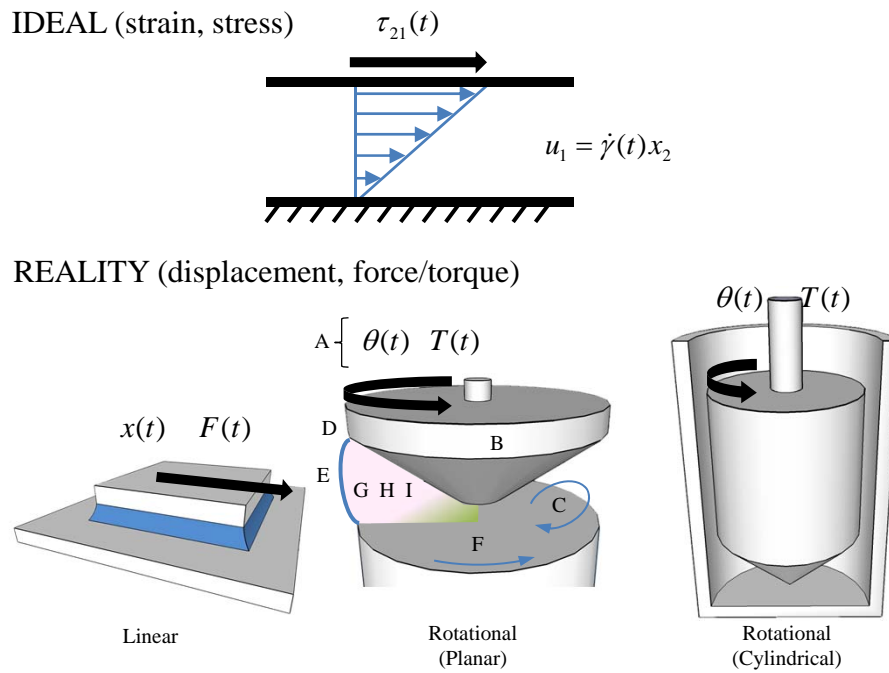
Fig. 1 Ideally, shear rheological properties are defined from strain \gamma(t) and stress \tau_{yx}(t) in homogeneous simple shear. In reality, boundary displacements and loads are measured and non-ideal experimental artifacts must be considered. The effects labeled as (A)-(I) are particularly important with biological complex fluids, and include (A) Resolution/range of measured load and displacement, (B) Instrument inertia (if load and displacement are measured on same boundary), (C) Fluid inertia and secondary flows, (D) Surface tension, (E) Free surface interfacial rheology, (F) Slip at boundaries, (G) Sample underfill or overfill, (H) Small volume and gap, (I) Non-homogenous sample from settling, migration, or rheotaxis.
