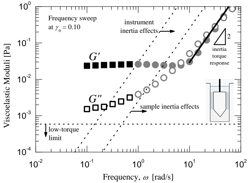
Fig. 6 Low-torque and instrument-inertia limits shown for oscillatory frequency sweep of hagfish gel. Low-torque limit from Eq. 14 with constant \gamma_0 ; instrument-inertia limit from Eq. 18; sample inertia limit from Eq. 26. The inertial torque response (solid line) is from Eq. 20 with \varepsilon = 0.01 being the error in the instrument inertia torque correction. Gray circles indicate when raw phase angle jumps from < 15^\circ to > 130^\circ which is also an indication that instrument inertia corrections must be made. (Data originally published in [5].)
