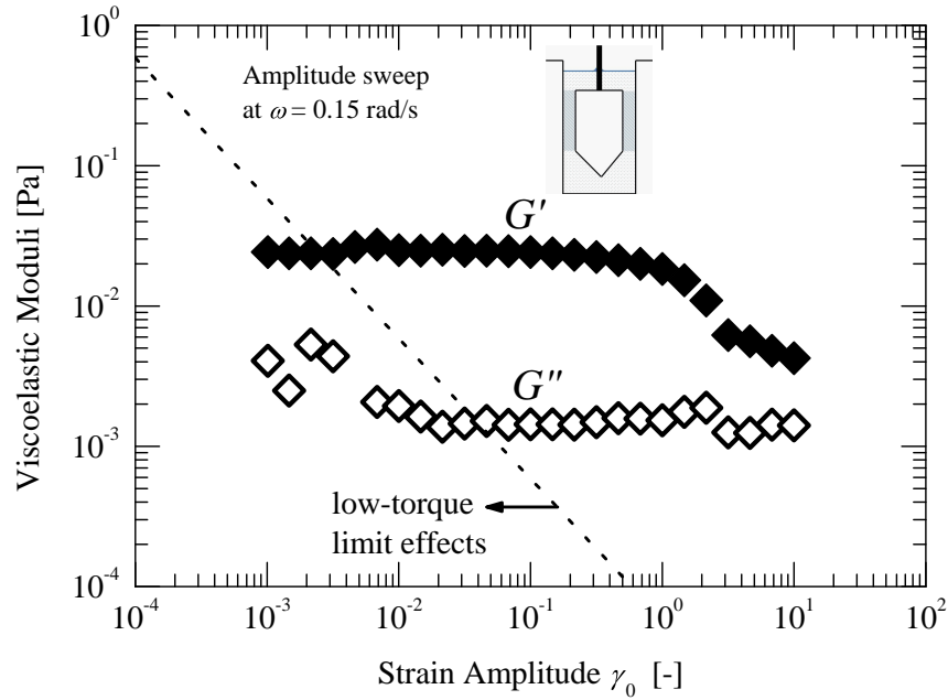
Fig. 5 Low-torque limit shown for oscillatory strain-amplitude sweep of hagfish gel. The experimental boundary helps identify the most believable data, and explains the increased measurement variability of G'' compared to G' at the same strain amplitude. Low-torque limit drawn from Eq. 14 using T_{\min} = 0.003 \mu\text{N.m} . (Data originally published in [5].)
