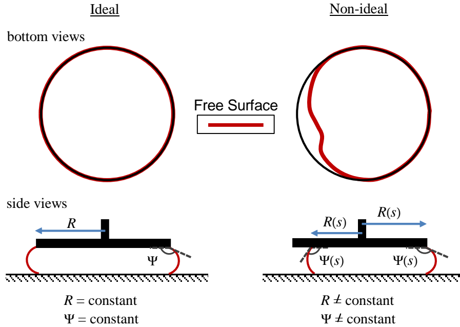
Fig. 9 Contact line and interface angle: ideal versus nonideal. Nonideal asymmetries are exaggerated compared to typical loading and can also occur as a result of overfilling. The nonideal condition may create artifacts of apparent shear thinning due to the presence of a constant surface tension torque. (Figure adapted from [13].)
