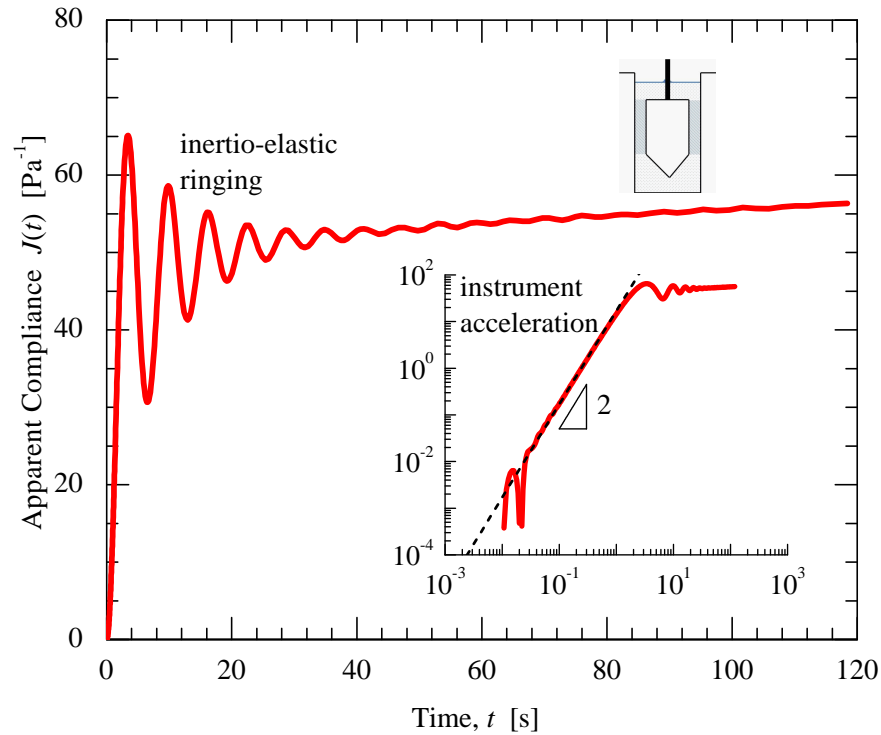
Fig. 7 Step torque test with hagfish gel in concentric cylinder geometry. Plotted as apparent compliance J(t) = F_\gamma \theta(t) / (F_\tau T_0) , showing instrument inertia effects: acceleration (inset) and inertio-elastic ringing. These effects can occur in rheometer designs where load is measured at the moving boundary. The acceleration can be predicted by Eq. 23, here using the value \frac{I F_\tau}{F_\gamma} = 2.9465 \cdot 10^{-2} \text{ Pa}\cdot\text{s}^2 . The ringing can be used to extract linear and nonlinear viscoelastic information as described in the text. Both effects obscure the true creep compliance of the material. (Data originally published in [14].)
