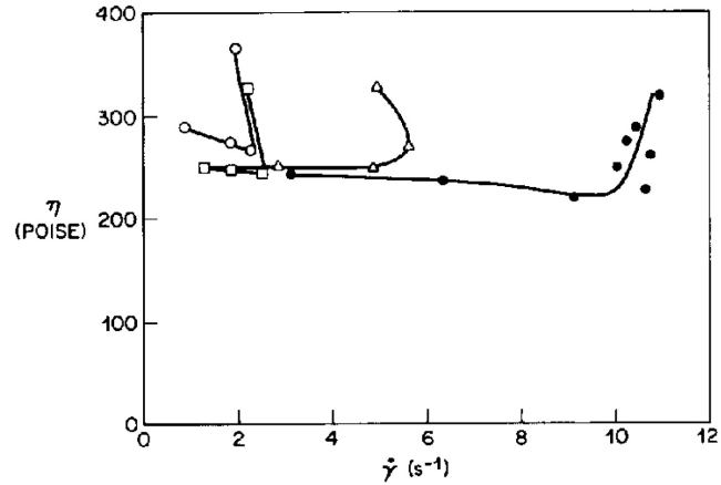
Fig. 8 Purely elastic instabilities cause apparent shear thickening of steady shear viscosity. Here with a dilute solution of polyisobutylene with nominal molecular weight 2.7 \cdot 10^6 from [27]. The thickening appears at a critical shear rate (Weissenberg number); the accessible range of experiments is extended by decreasing the gap, here with a parallel disk geometry at different gaps ranging from 2 mm (open circles) to 0.3 mm (filled circles). (Reprinted from Magda & Larson [27], Journal of Non-Newtonian Fluid Mechanics , Fig. 10, Copyright (1988), with permission from Elsevier.)
