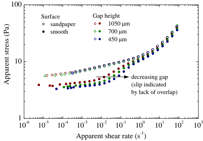
Fig. 13 Slip behavior on a smooth geometry surface can decrease flow stress and cause inconsistent gap-dependence, as shown here for Nivea Lotion tested with different surfaces and gaps using parallel disks of diameter D = 40 mm. A sandpaper surface eliminates slip artifacts, showing superposed data for different gap heights. (Previously unpublished work of author RHE.)
