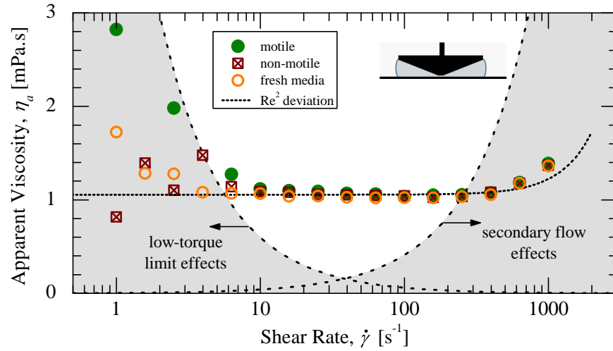
Fig. 3 Steady shear flow measurements could be misinterpreted as shear-thinning and shear-thickening if an experimental window is not identified. Here, shown with dilute suspensions of motile and non-motile swimming microalgae Dunaliella primolecta compared to fresh media (no cells present). The low-torque limit, described in Section 3.1, is drawn from Eq. 13 using T_{\min} = 0.1 \mu\text{N.m} . The secondary flow limit, described in Section 3.3, is drawn from Eq. 31 using \text{Re}_{\max} = 4 . The \text{Re}^2 line is from the expected increase in torque due to secondary flow, Eq. 29. (Previously unpublished work of authors RHE and LMC.)
