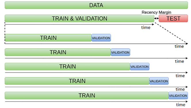
Fig. 2. Increasing-window CrossValidation.
