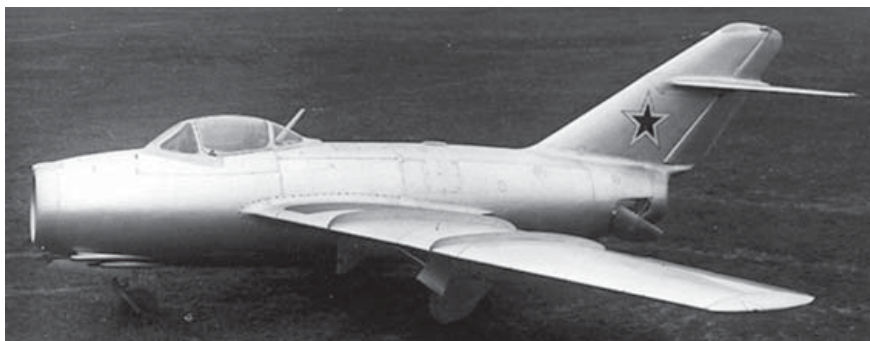
The first MiG-15 of the small initial production batch – designated the MiG-15(S) by the MiG OKB – during acceptance trials. Note the small speedbrake (extended) added to the tailpipe almost as an after-thought. [FoxbatFiles.com]
