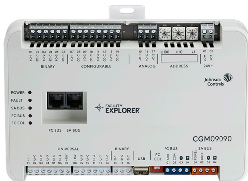
Figure 1: FX-CGM09090 General Purpose Application Controller
