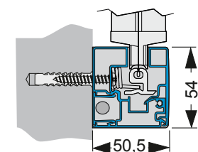
Wall attachment of lateral tracks (top view)
