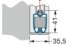
Wall attachment of lateral tracks (top view)
