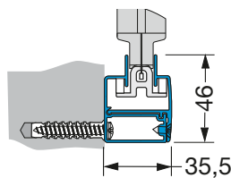
Wall attachment of lateral tracks (top view)
