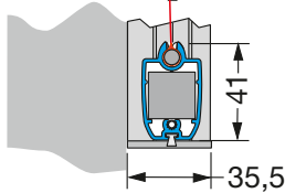
Wall attachment of lateral tracks (top view)
