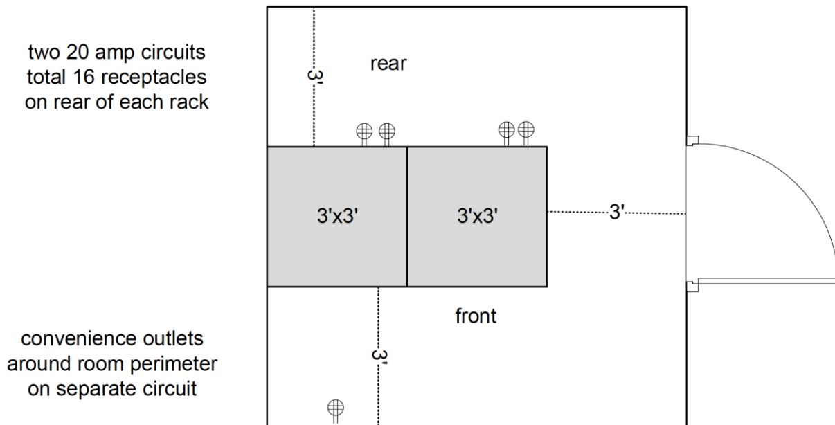
Typical Telecommunications Room (Additional space must be added for wall-mounted equipment such as card access panels.)
