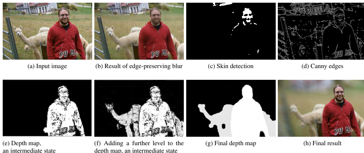
Figure 3: Results of various intermediate steps of our pipeline. Input image (a) was captured at 27 mm full-frame equivalent at f/2.8 on a compact camera with crop factor 5.5. The binary foreground–background segmentation mask is in Fig. (g), final result with bokeh effect applied is in (h).
