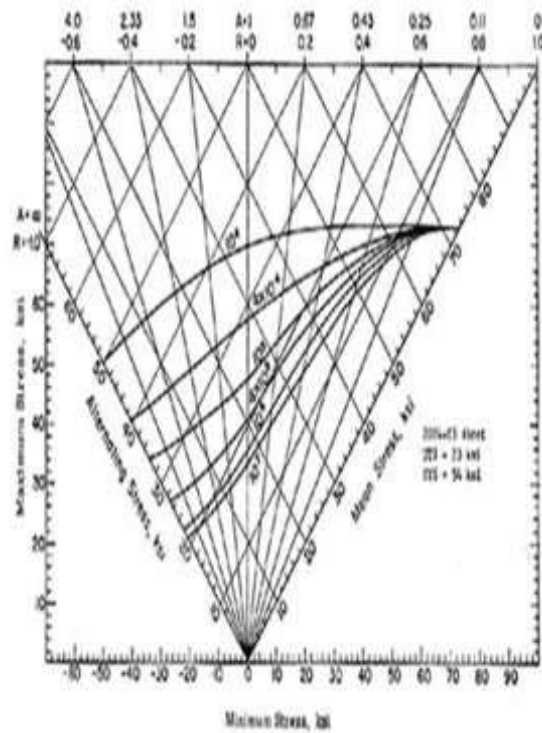
Figure 8.1: S-N curve
