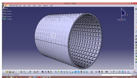
Fig 5.1 Fuselage Model
