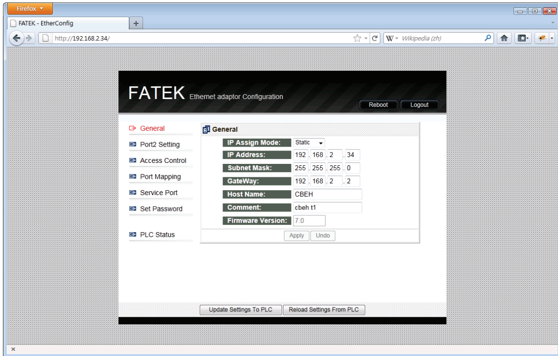
Configuration setup for CBEH board
