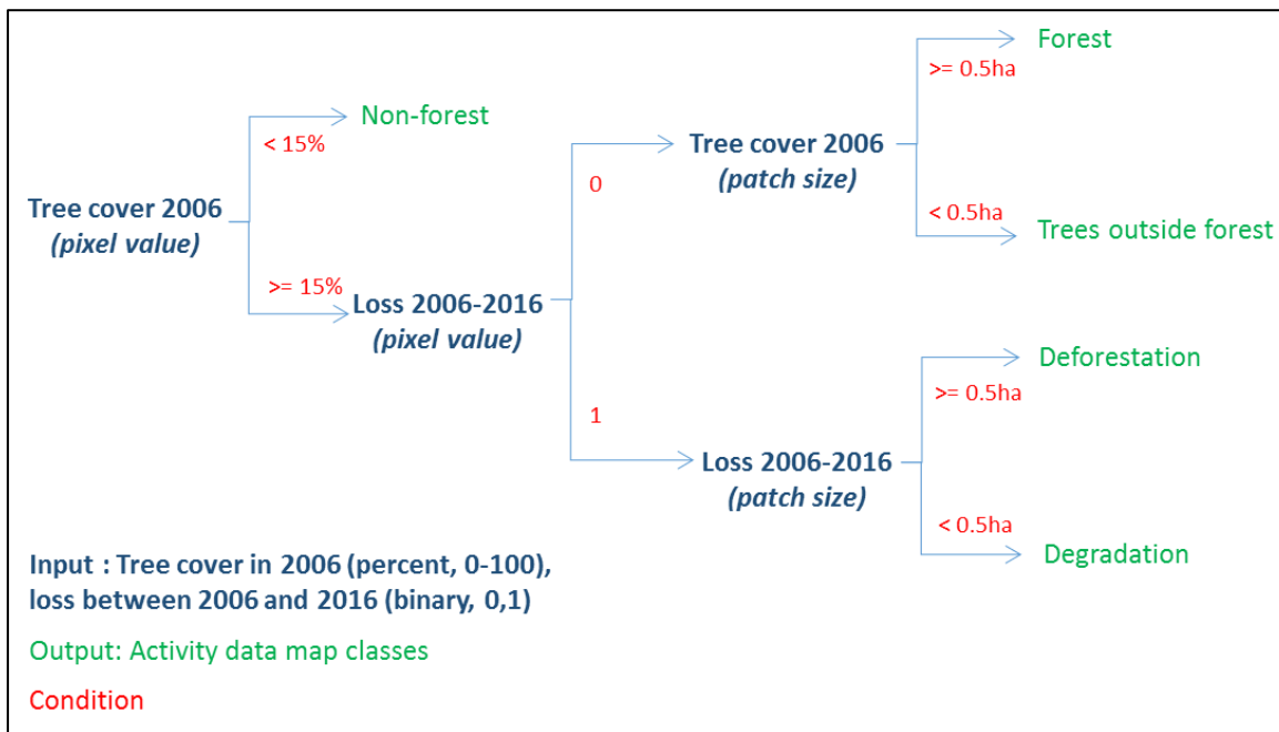
Figure 6 Decision tree for the creation of the forest change map
