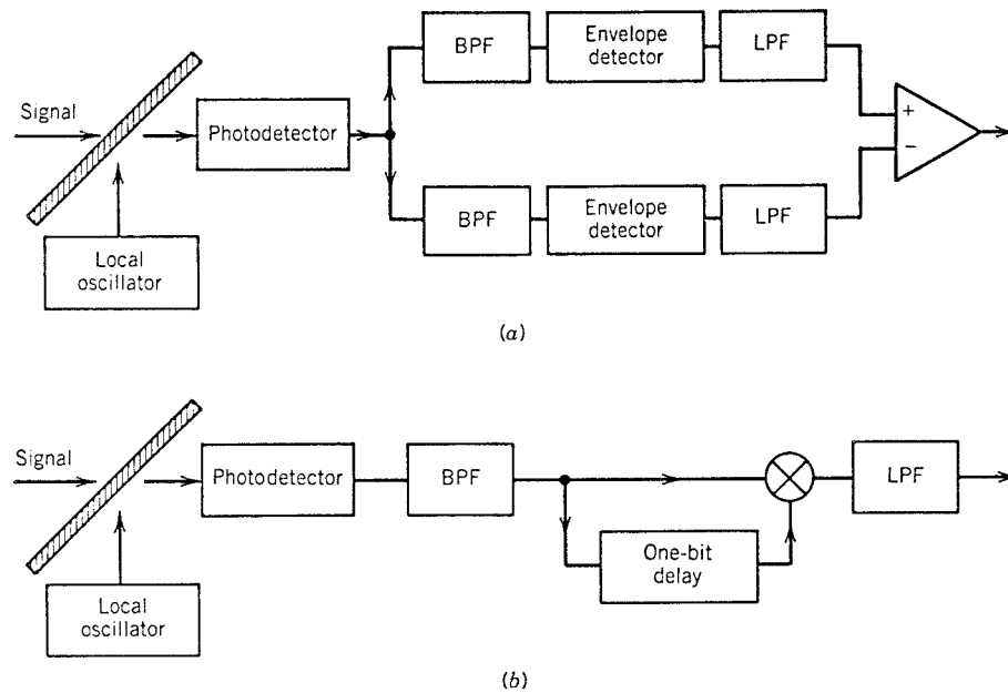
Figure 10.6: (a) Dual-filter FSK and (b) DPSK asynchronous heterodyne receivers.
