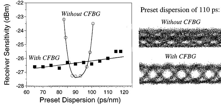
Figure 7.18: Receiver sensitivities measured in a 160-Gb/s experiment as a function of the preset dispersion with (squares) and without (circles) a chirped fiber-Bragg grating (CFBG). The improvement in the eye diagram is shown for 110 ps/nm on the right. (After Ref. [165]; ©2000 IEEE; reprinted with permission.)
