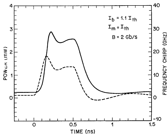
Figure 3.22: Simulated modulation response of a semiconductor laser to 500-ps rectangular current pulses. Solid curve shows the pulse shape and the dashed curve shows the frequency chirp imposed on the pulse ( \beta_c = 5 ).
