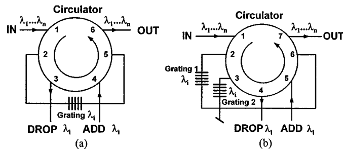
Figure 8.13: (a) Two designs of add-drop multiplexers using a single optical circulator in combination with fiber gratings. (After Ref. [94]; ©2001 IEEE; reprinted with permission.)
