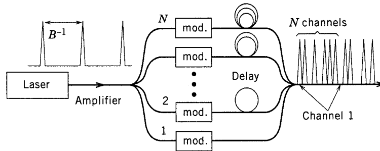
Figure 8.26: Design of an OTDM transmitter based on optical delay lines.
