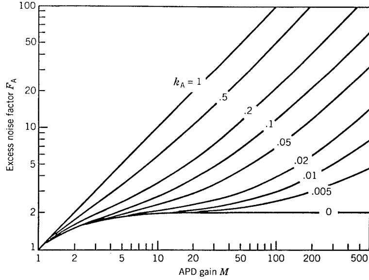
Figure 4.16: Excess noise factor F_A as a function of the average APD gain M for several values of the ionization-coefficient ratio k_A .
