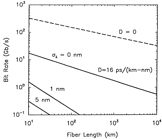
Figure 2.13: Limiting bit rate of single-mode fibers as a function of the fiber length for \sigma_\lambda = 0, 1, and 5 nm. The case \sigma_\lambda = 0 corresponds to the case of an optical source whose spectral width is much smaller than the bit rate.
