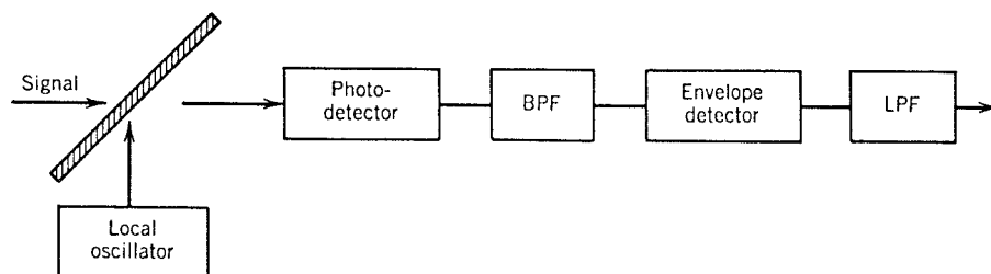
Figure 10.5: Block diagram of an asynchronous heterodyne receiver.
