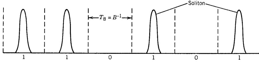
Figure 9.5: Soliton bit stream in RZ format. Each soliton occupies a small fraction of the bit slot so that neighboring solitons are spaced far apart.
