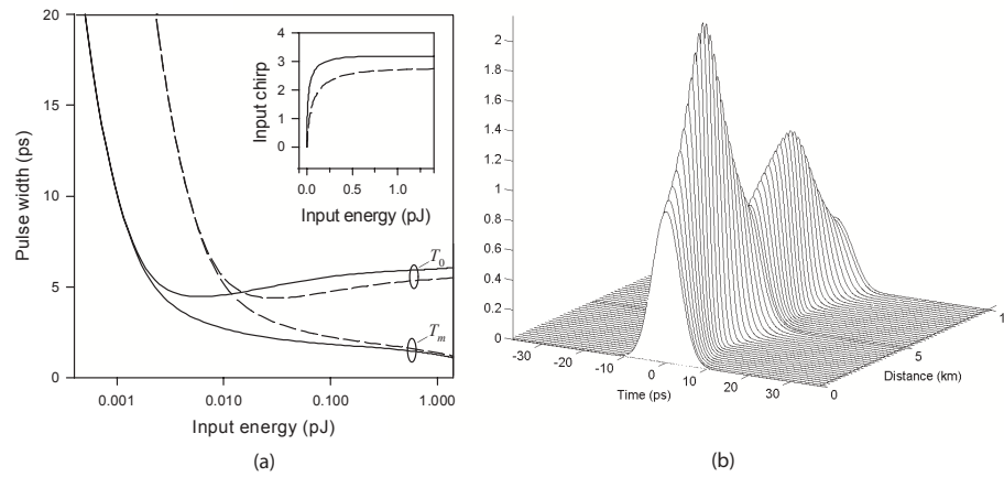
Figure 9.15: (a) Changes in T_0 (upper curve) and T_m (lower curve) with input pulse energy E_0 for \alpha = 0 (solid lines) and 0.25 \text{ dB/km} (dashed lines). The inset shows the input chirp C_0 in the two cases. (b) Evolution of the DM soliton over one map period for E_0 = 0.1 \text{ pJ} and L_A = 80 \text{ km} .
