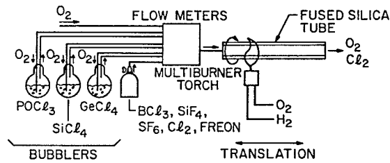
Figure 2.21: MCVD process commonly used for fiber fabrication. (After Ref. [87]; ©1985 Academic Press; reprinted with permission.)
