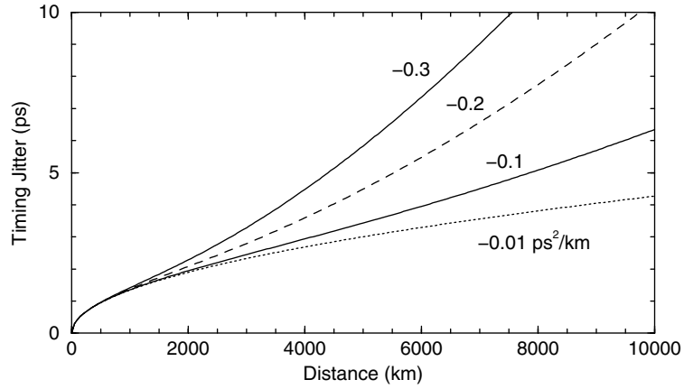
Figure 6.23: ASE-induced timing jitter as a function of system length for several values of the average dispersion \beta_2 .
