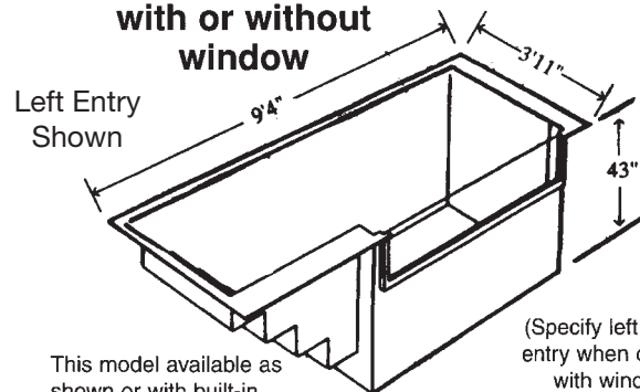
Model 13-A with or without window
