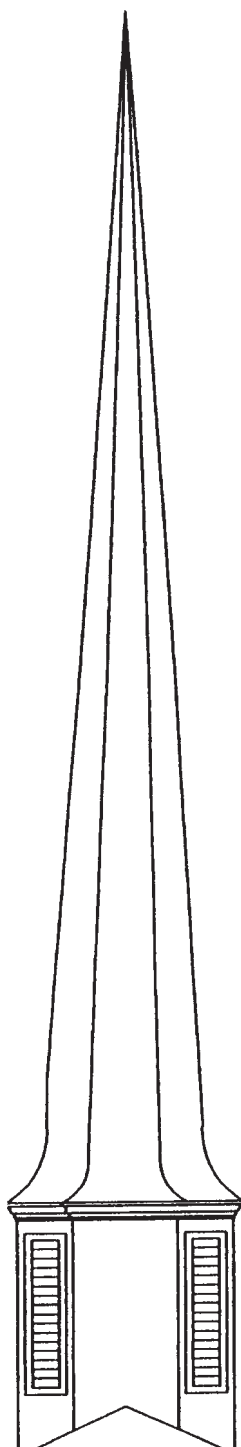
Model # 325 32'5" High 5'0" Base (Windows & louvers available, cross optional)
