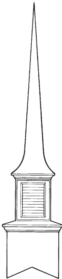
Model # 330 24' High 4'6" Base
