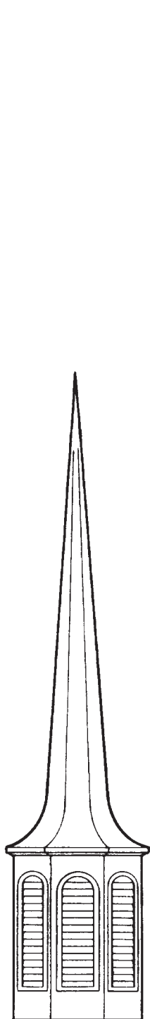
Model # 300 21'0" High 48" Base
