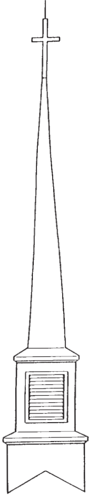
Model # 275 24'10" High 4'0" Base (Shown with 3' optional cross)
