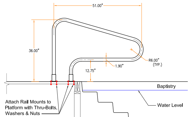
51-Inch Deck Mounted Commercial Stair Rail
