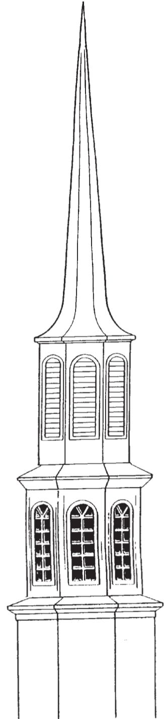
Model # 628 35' High 7'9" Octagon Base Krinklglas Optional
