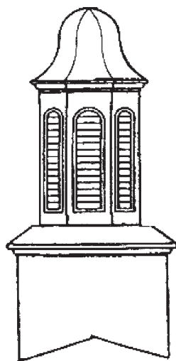
Model # C295 11' High 3'9" Base
