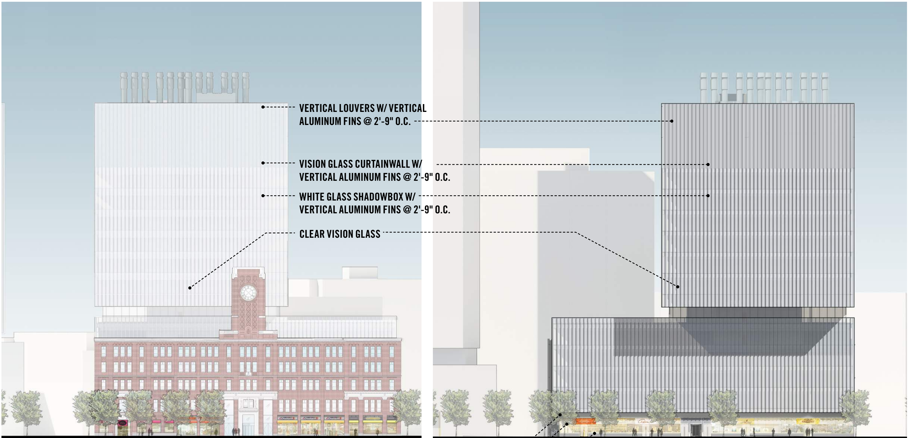
NORTH ELEVATION - MATERIALS
