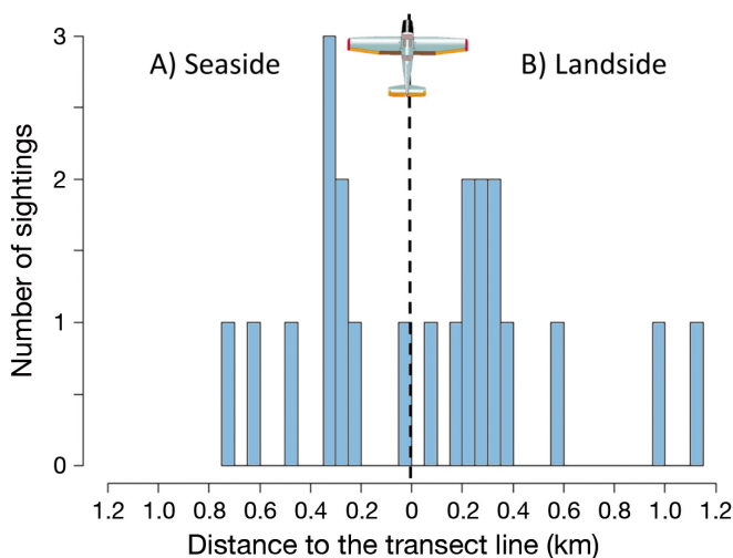
Fig. 6. Distance between the plane and sighting locations of white whales during an aerial survey conducted in the Svalbard Archipelago, summer 2018
