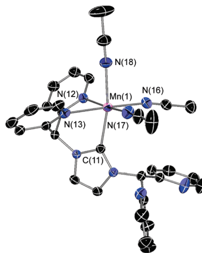
Figure 8. X-ray crystal structure of [( \kappa^3 -PY4Im)Mn(MeCN) 3 ] 2+ , as observed in 9. Thermal ellipsoids are shown at 50% probability, hydrogen atoms omitted for clarity. Selected bond lengths (Å) and angles (deg): Mn(1)–C(11) 2.213(2); Mn(1)–N(12) 2.2625(17); Mn(1)–N(13) 2.3062(18); Mn(1)–N(16) 2.251(2); Mn(1)–N(17) 2.1917(19); Mn(1)–N(18) 2.253(2); C(11)–Mn(1)–N(12) 84.27(7); C(11)–Mn(1)–N(13); 80.62(7); C(11)–Mn(1)–N(16) 96.22(7); C(11)–Mn(1)–N(17) 101.32(7); C(11)–Mn(1)–N(18) 167.95(7).
