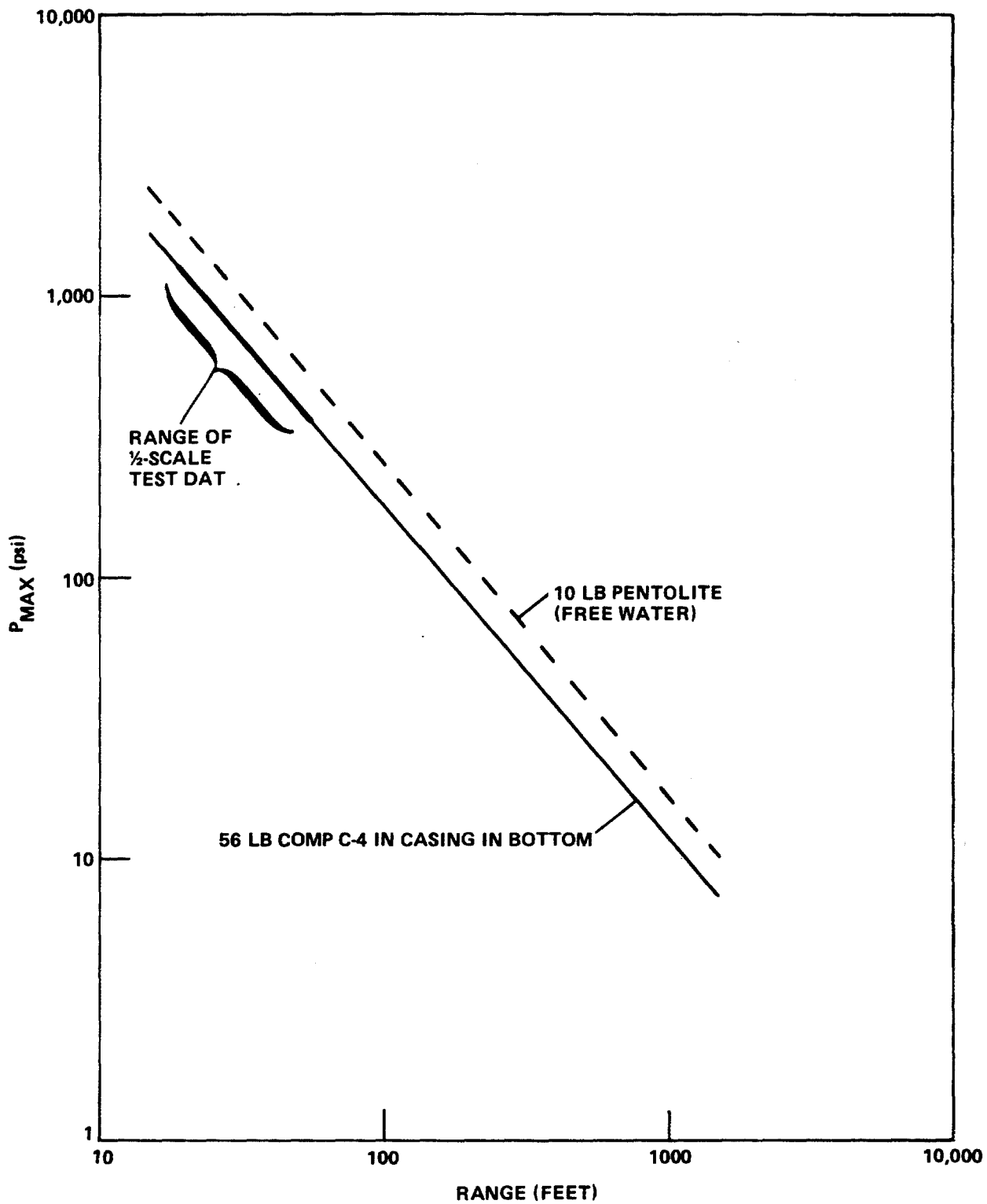
FIGURE 3-4 P_{MAX} — COMPARISON OF EQUATION FOR 56-LB SEVERANCE EXPLOSION WITH 10-LB FREE-WATER EXPLOSION
