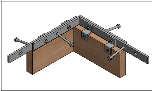
Steel Edge Nosing w/ Clip - 2-Way Intersection
