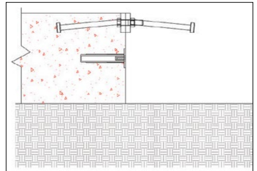
Step 3: Remove Wood Form and Fastener Clip.
