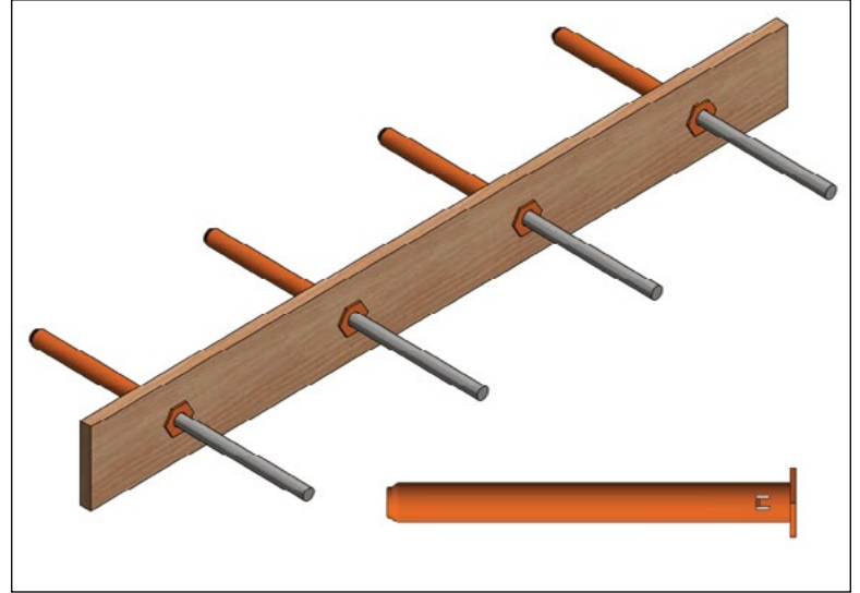
Plastic sleeves are used with predrilled expansion boards, like cedar or polypropylene, to accurately position and align smooth steel dowels in the adjoining concrete section.
