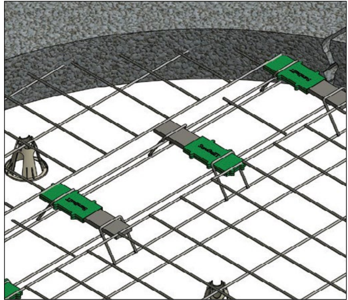
The labor-saving 12' SureDowel Basket is placed as a single unit at every planned concrete joint, along with typical chairs and reinforcement.
