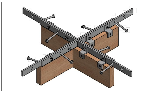
Steel Edge Nosing w/ Clip - 4-Way Intersection
