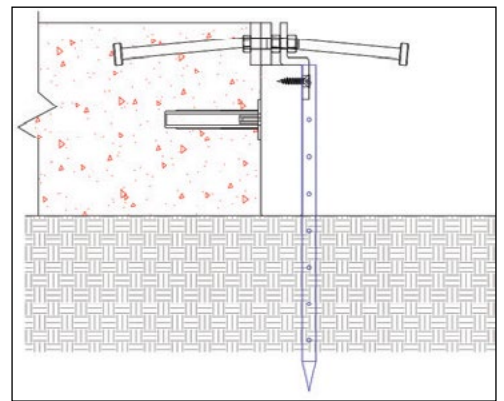
Step 2: Place Taper Sleeve in Form, Pour Concrete one side.
