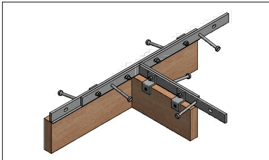
Steel Edge Nosing w/ Clip - 3-Way Intersection
