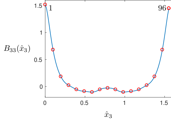
Figure T.4: Periodic two-point correlation, B_{33}(\hat{x}_3) = \langle v'_3(x_3)v'_3(x_3 + \hat{x}_3) \rangle , of DNS data in channel flow taken from [100].
