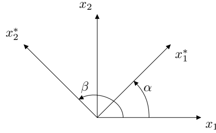
Figure AA.1: Transformation between the coordinate systems (x_{1*}, x_{2*}) and (x_1, x_2) .
