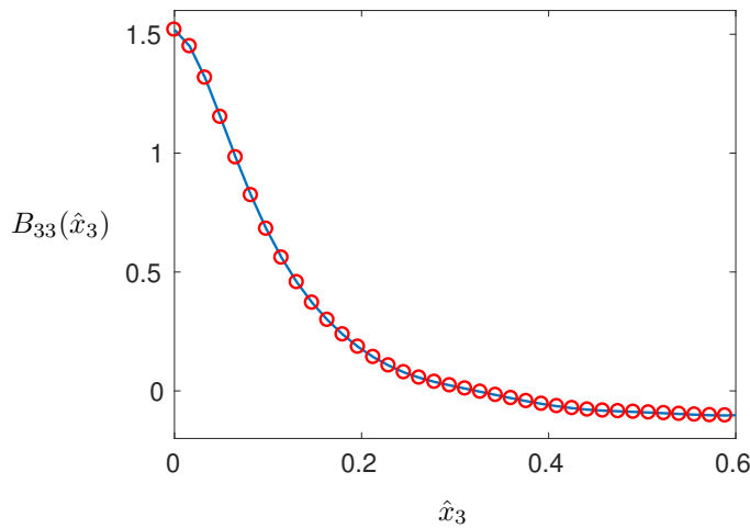
Figure T.1: Two-point correlation, B(\hat{x}_3) = \langle v'_3(x_3 - \hat{x}_3)v'_3(x_3) \rangle , of DNS data in channel flow taken from [100].
