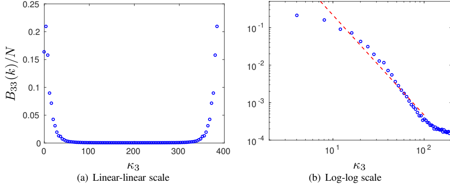
Figure T.5: The energy spectrum of \overline{v_3'^2} versus wavenumber, \kappa_3 . Dashed line in b) show -5/3 slope. Taken from [100].
