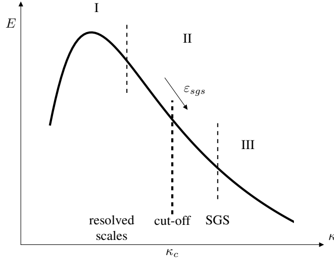
Figure S.3: Spectrum with cut-off.
