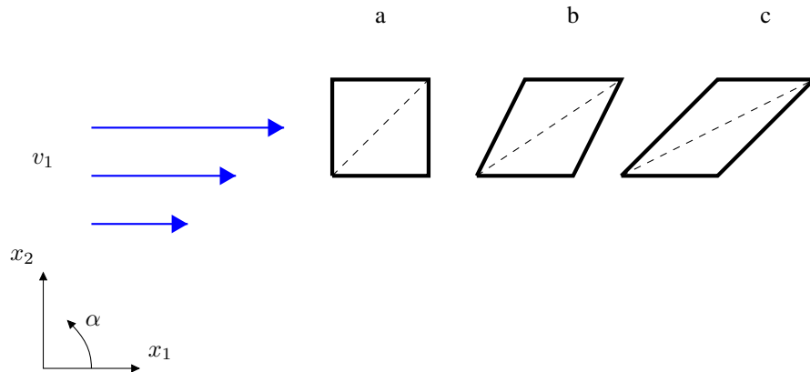
A shear flow. A fluid particle with vorticity. v_1 = cx_2^2 .
