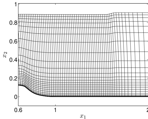
Figure V.1: Hump flow. Grid. Every 4 th grid line is shown.
