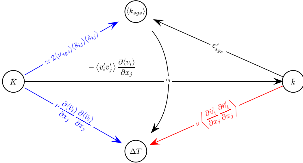
Figure S.4: Transfer of kinetic turbulent energy. \bar{K} = \frac{1}{2}\langle\bar{v}_i\rangle\langle\bar{v}_i\rangle and \bar{k} = \frac{1}{2}\langle\bar{v}'_i\bar{v}'_i\rangle denote time-averaged kinetic and resolved turbulent kinetic energy, respectively. \Delta T denotes increase in internal energy, i.e. dissipation. The cascade process assumes that the term in red is negligible (see also Fig. 8.2). The terms in blue show viscous and the SGS dissipation of the mean flow which is not included in the cascade process.
