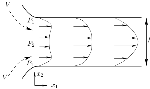
Flow in a horizontal channel. The inlet part of the channel is shown.
