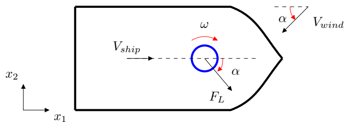
Flettner rotor (in blue) on a ship. The relative velocity between the ship and the wind is V_{wind} + V_{ship} . The ship moves with speed V_{ship} . Top view.
