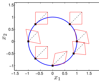
Ideal vortex.
