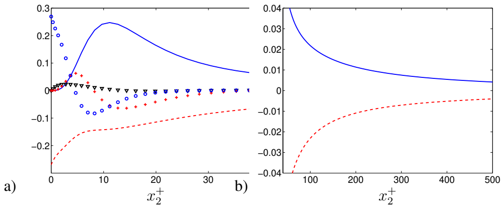
a) Zoom near the wall; b) Outer region. —: P^k ; - - : -\epsilon ; \nabla : -\partial \overline{v' p'} / \partial x_2 ; +: -\partial \overline{v'_2 v'_i v'_i} / 2 / \partial x_2 ; \circ : \nu \partial^2 k / \partial x_2^2 .
