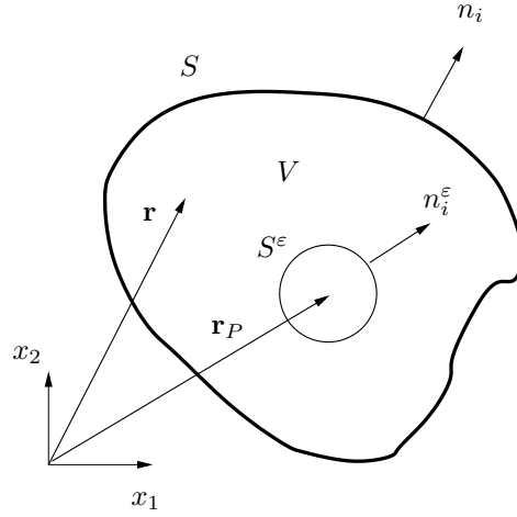
Figure AB.1: Green's third formula. A volume V with bounding surface S with normal vector n_i . In V there is a small sphere S^\epsilon located at \mathbf{r}_P with radius \epsilon and normal vector n_i^\epsilon .
