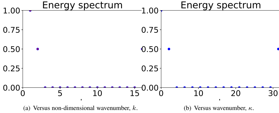
Figure T.3: The U/N Fourier coefficients.
