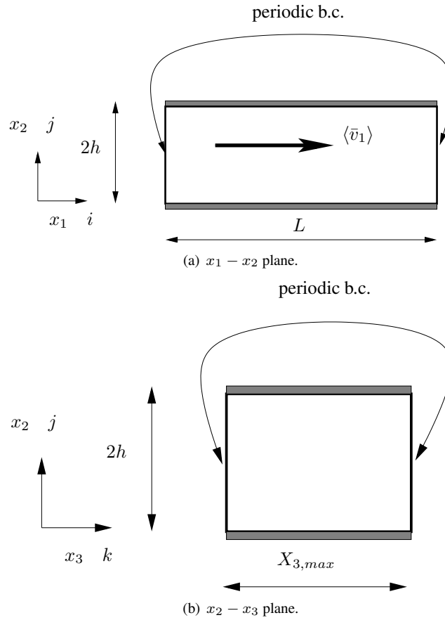
Figure S.1: Channel domain.
