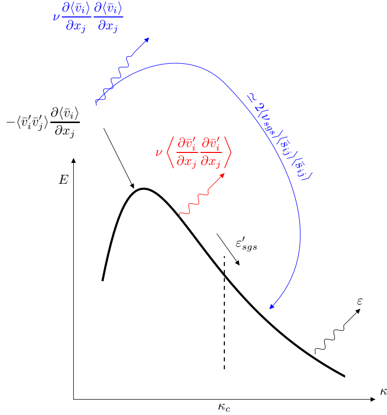
Figure S.5: Energy spectrum. Transfer of kinetic energy. The cascade process assumes that the term in red is negligible (see also Fig. 8.2). The terms in blue show viscous and the SGS dissipation of the mean flow which is not included in the cascaded process.
