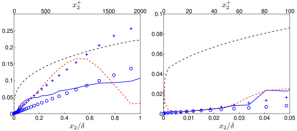
Figure 22.4: Turbulent length scales in fully developed channel flow. Hybrid LES-RANS. Left: global view; right: zoom. 32 \times 64 \times 32 mesh. Re_\tau = 2000 . \Delta x_1/\delta = 0.39 , \Delta x_3/\delta = 0.19 , x_2 -stretching of 17%. — : \langle L_{vK,inst} \rangle ; - - : L_{vK,steady} ; - - - : (\Delta x_1 \Delta x_2 \Delta x_3)^{1/3} ; \circ : \Delta x_2 ; +: \ell_{k-\omega} = k^{0.5}/(c_\mu^{1/4} \omega) .
