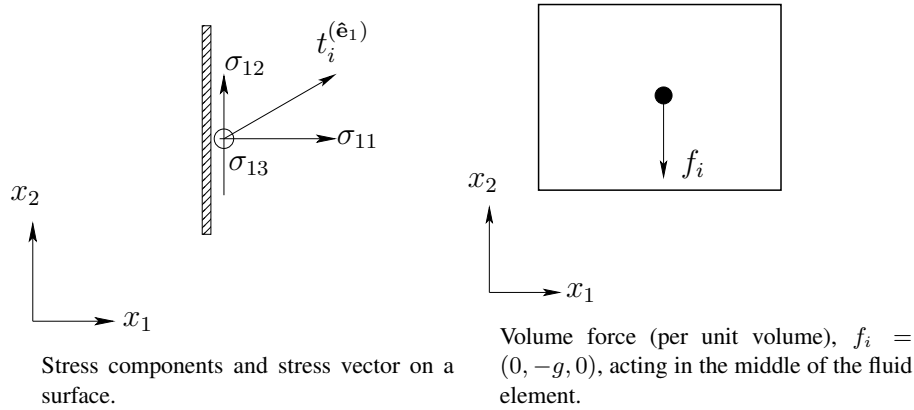
Stress tensor, volume (gravitation) force and stress vector, t_i^{(\hat{e}_1)} .
