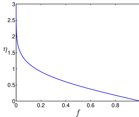
The velocity, f = v_1/V_0 .
