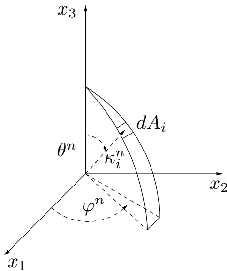
Figure O.1: The probability of a randomly selected direction of a wave in wave-space is the same for all dA_i on the shell of a sphere.
