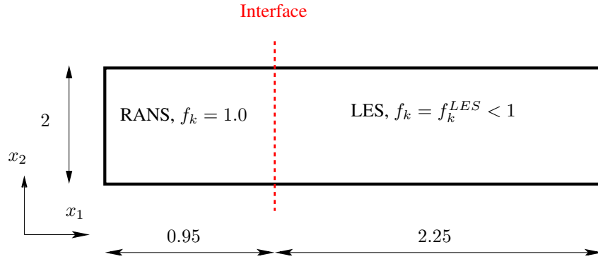
Figure W.1: Channel flow configuration. The interface separates the RANS and the LES regions.
