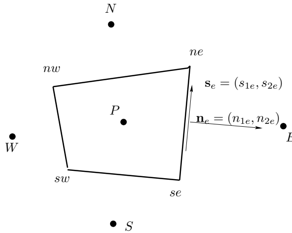
Figure R.1: Control volume. The velocity v_1 is stored at the corners ( ne, nw, \dots ). Coordinates x_1, x_2 are given at the corners ( ne, nw, \dots ).
