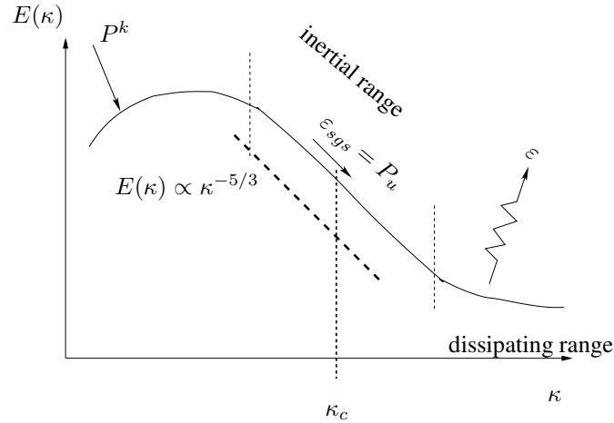
Figure W.2: Energy spectrum.
