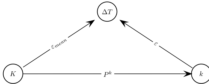
Figure A.4: Transfer of energy between mean kinetic energy ( K ), turbulent kinetic energy ( k ) and internal energy (denoted as an increase in temperature, \Delta T ). K = \frac{1}{2}\bar{v}_i\bar{v}_i and k = \frac{1}{2}\overline{v'_i v'_i} .
