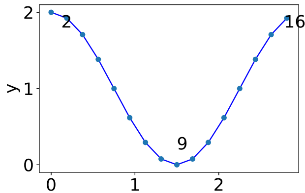
Figure T.2: The u function.
