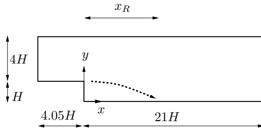
Figure S.2: Backstep domain.
