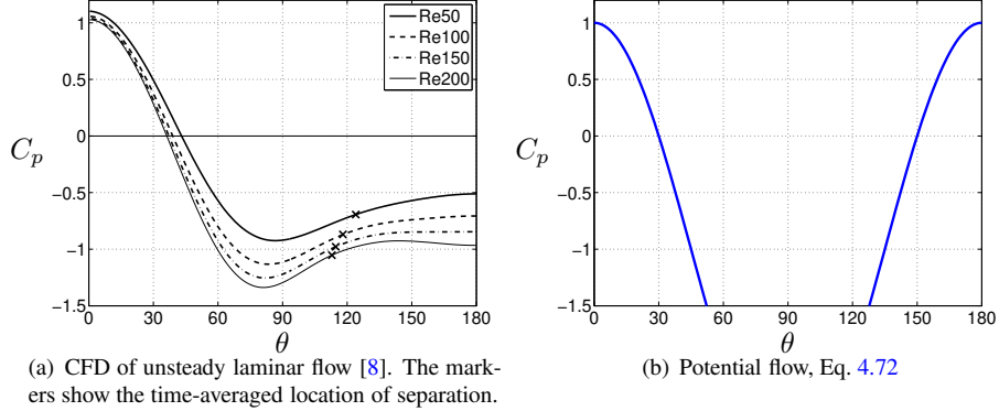
Figure 4.13: Pressure coefficients.
