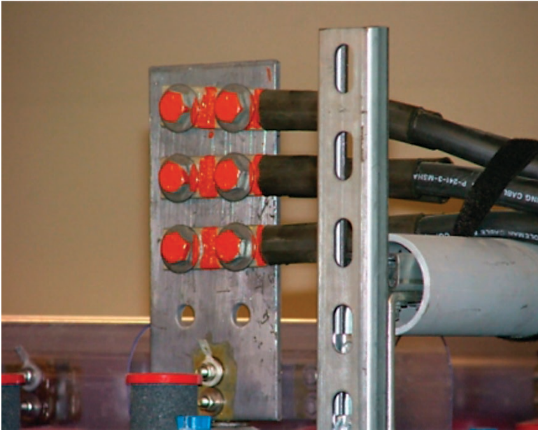
Simple painted markings like these are often used for high-emissivity “targets” that dramatically increase the reliability of radiometric measurements.
