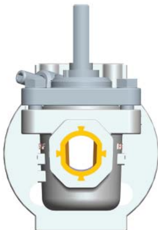
Dovetail Liner Section Pictured with EZ-SEAL® Cover (Optional)
