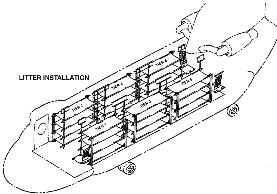
Figure A-2. CH-47D litter configuration
