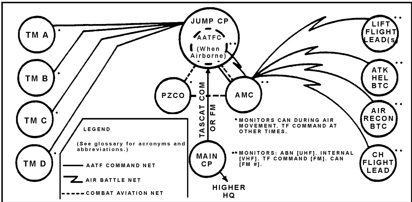
Figure 3-2. Air assault radio nets
