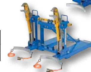
model FMDL-2
