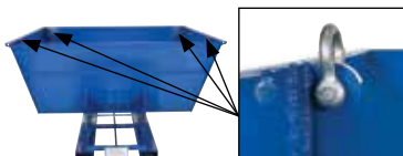
LIFTING LUGS
