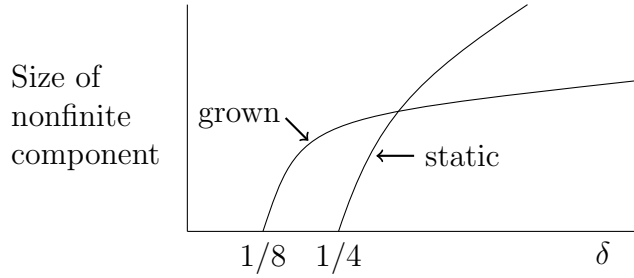
FIGURE 3.14: Comparison of the static random graph model and the growth model. The curve for the growth model is obtained by integrating g' .
