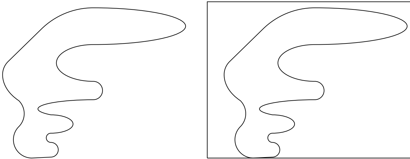
FIGURE 5.9: Area enclosed by curve.
