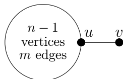
FIGURE 5.18: A connected graph consisting of n - 1 vertices and m edges along with a single edge (u, v) .
