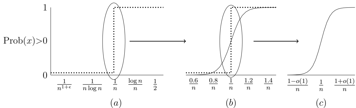
FIGURE 3.5: Figure 3.5(a) shows a phase transition at \frac{1}{n} . The dotted line shows an abrupt transition in \text{Prob}(x) > 0 from 0 to 1. For any function asymptotically less than \frac{1}{n} , \text{Prob}(x) > 0 is zero and for any function asymptotically greater than \frac{1}{n} , \text{Prob}(x) > 0 is one. Figure 3.5(b) expands the scale and shows a less abrupt change in probability unless the phase transition is sharp as illustrated by the dotted line. Figure 3.5(c) is a further expansion and the sharp transition is now more smooth.
