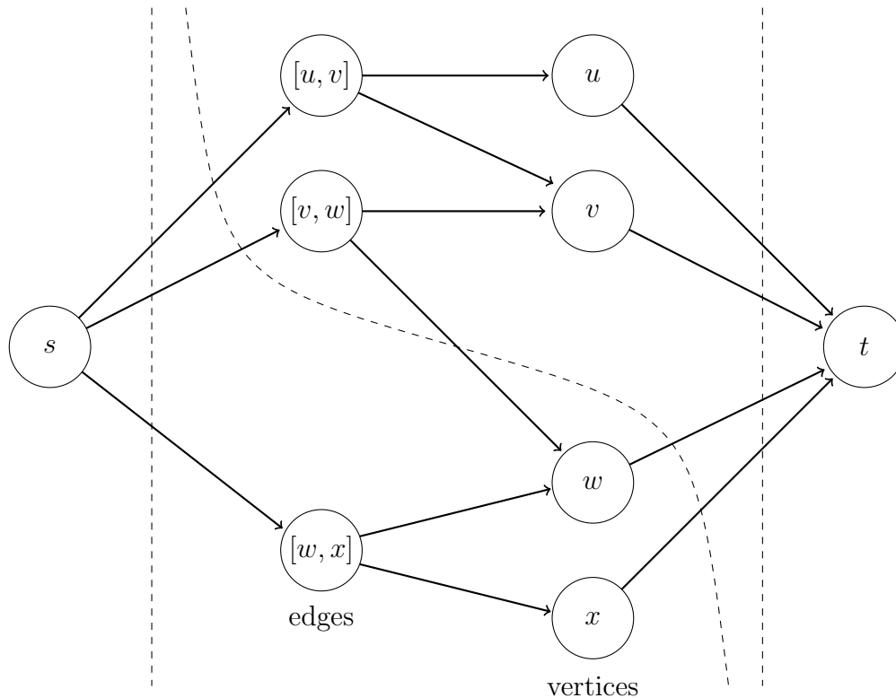
FIGURE 8.5: The directed graph H used by the flow technique to find a dense subgraph subset. For different values of \lambda in the above range there maybe different nontrivial cuts.
