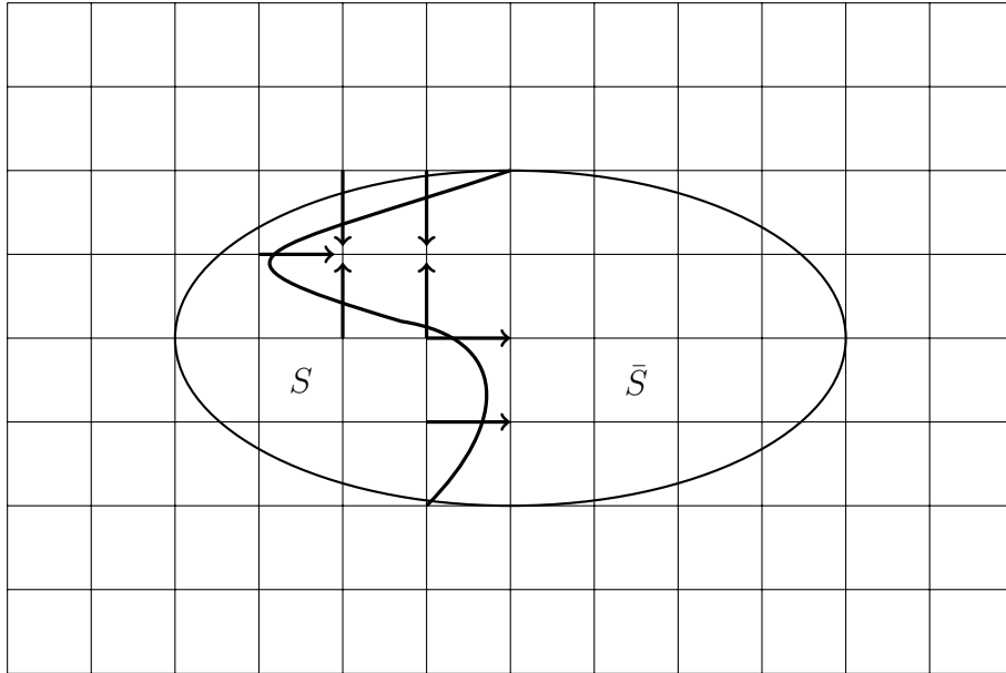
FIGURE 5.10: Each grid point in the ellipse is a state. The set of states in the ellipse is divided into two sets, S and \bar{S} , by the curve. The transitions from S to \bar{S} , which contribute to \Phi(S) , are marked with arrows.
