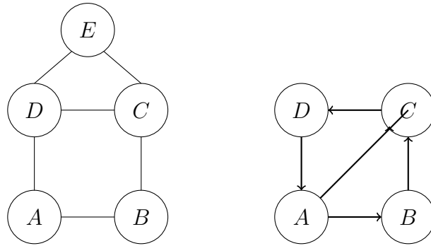
FIGURE 5.19: An undirected and a directed graph.
