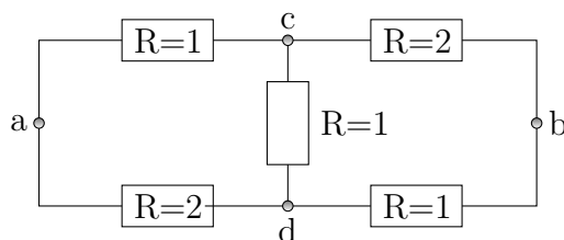
FIGURE 5.15: An electrical network of resistors.
