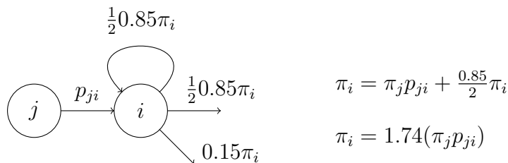
FIGURE 5.8: Impact on page rank of adding a self loop
