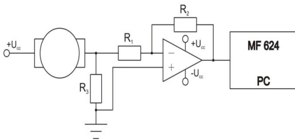
Figure 5. Wiring scheme
