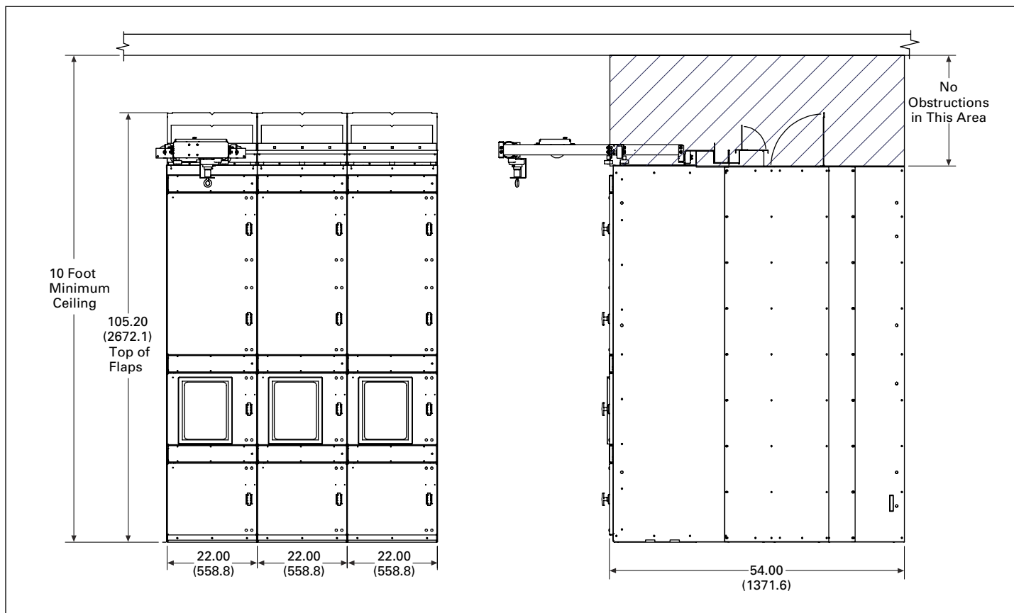
Figure 20.4-7. Non-Plenum Top Exit Configuration—Dimensions in Inches (mm)
