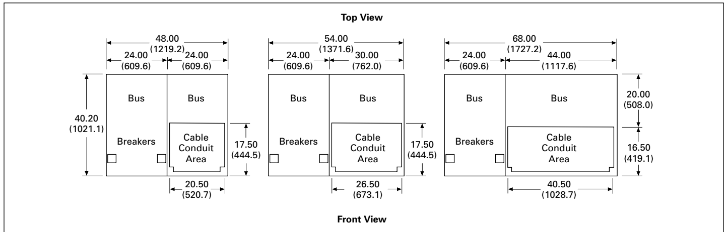
Figure 20.4-6. Floor Plans and Available Conduit Space—Front-Access Structures—Dimensions in Inches (mm)
