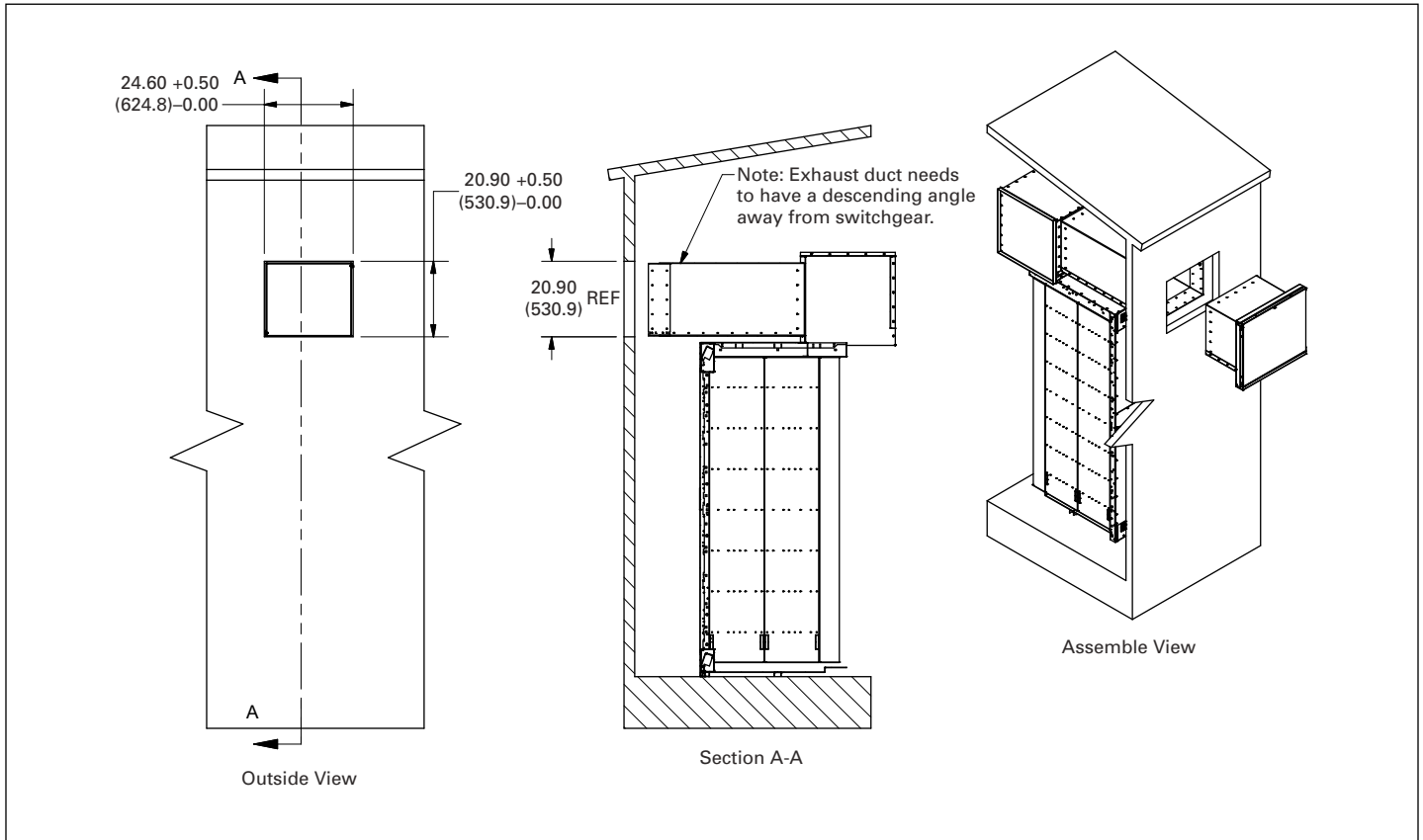
Figure 20.4-10. Wall Mounted Plenum Cutout Size and Location
