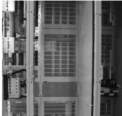
Optional Bus Compartment and Vertical Section Barriers
