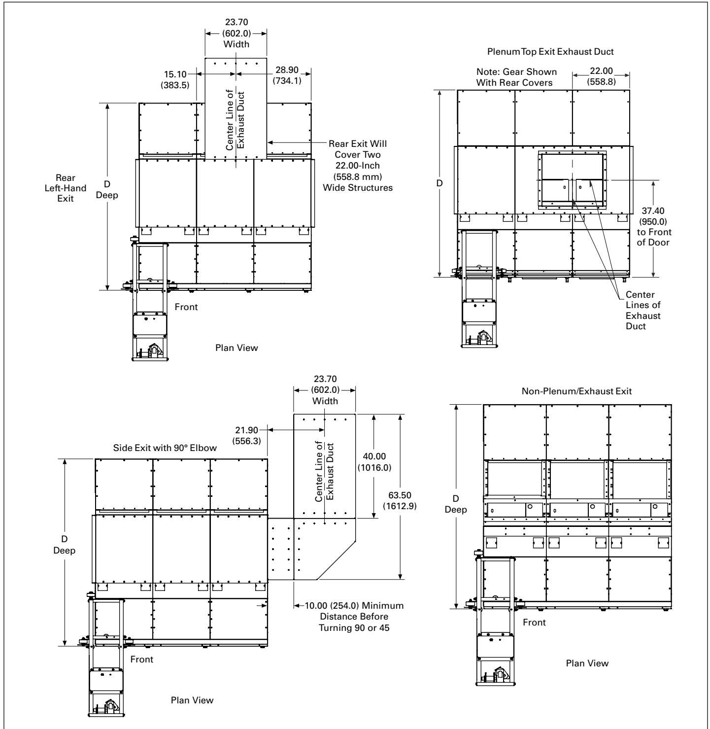
Figure 20.4-9. Arc-Resistant Switchgear Exhaust Configurations (Continued)
