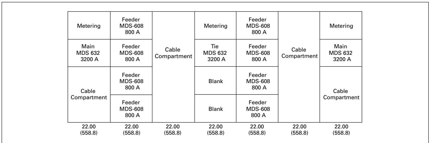
Figure 20.4-5. Front-Accessible Standard Breakers Main-Tie-Main Typical Layout—Dimensions in Inches (mm)
