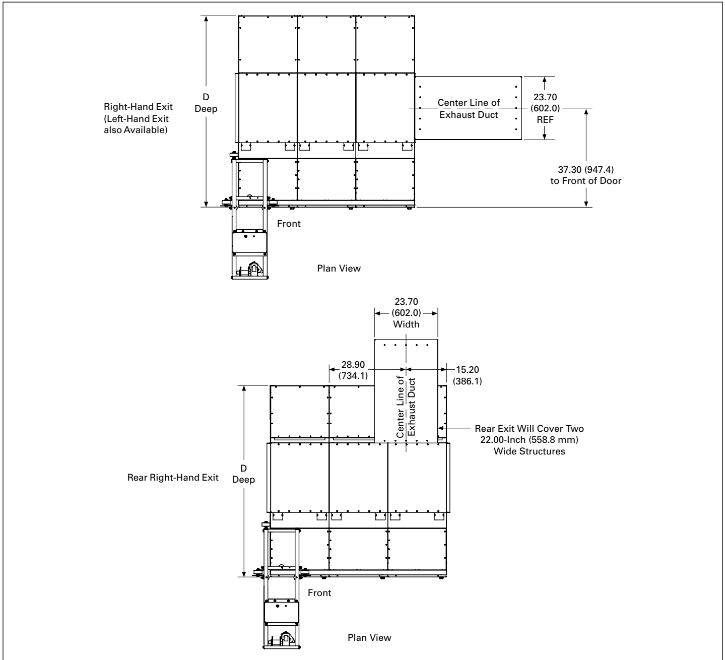
Figure 20.4-9. Arc-Resistant Switchgear Exhaust Configurations—Dimensions in Inches (mm)
