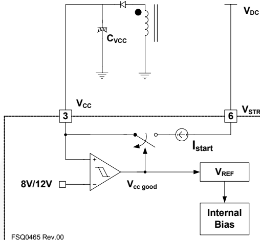
Figure 22. Startup Circuit
