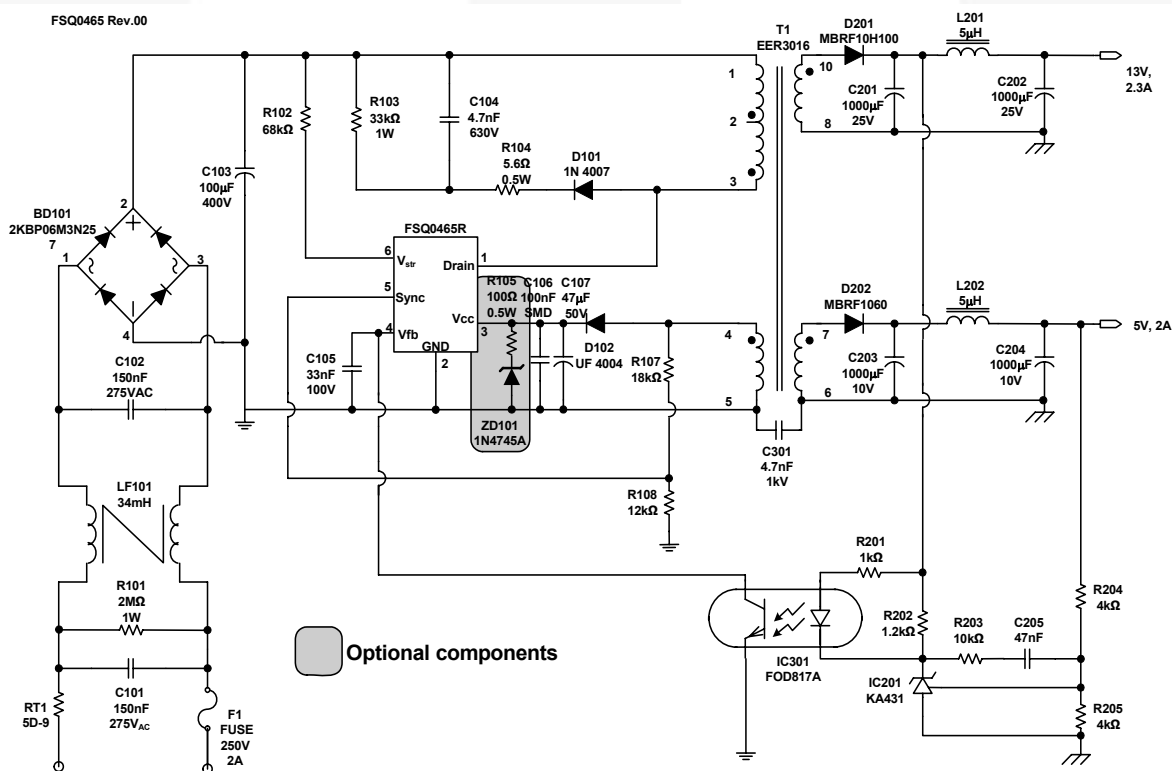
Figure 37. Demo Circuit of FSQ0465RS
