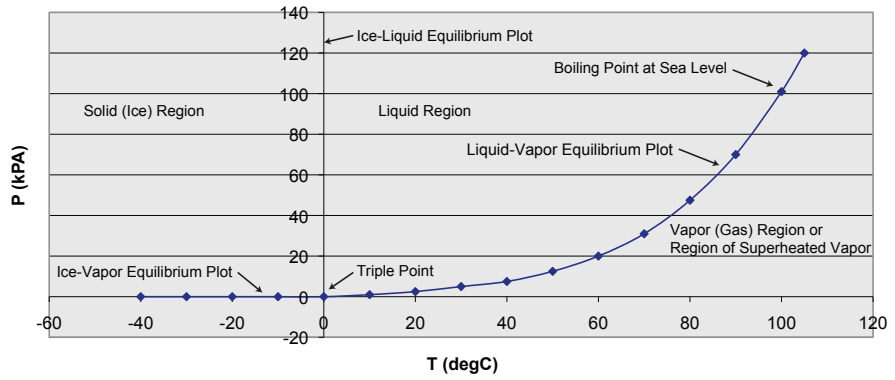
Figure 2.1 P-T Diagram for Water
