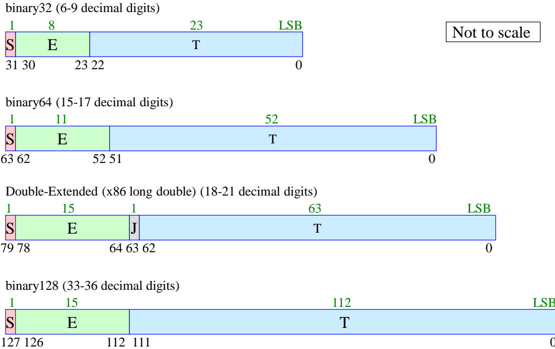
Figure 14.1 Common floating point formats, with S, E, T fields named as in [IEEE-754 p9]. (However, IEEE-754 numbers the bits from 0 on the left.)
