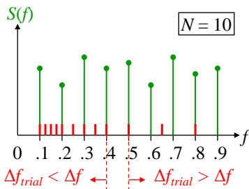
Figure 11.12 Nonuniformly spaced trial frequencies.
