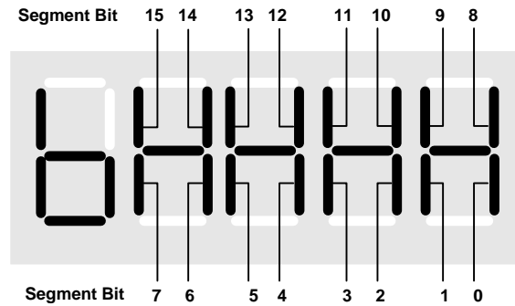
Fig. 1-3 Seven-segment display
