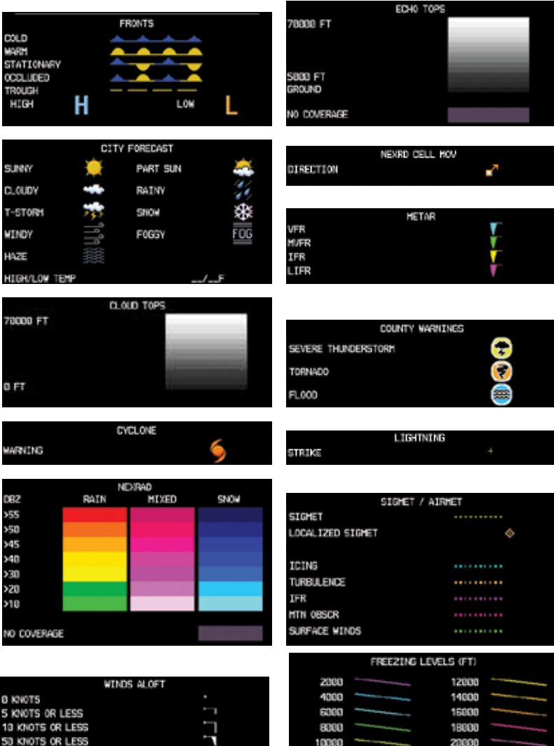
Figure 4-23 Weather Legends
