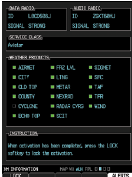
Figure 3-81 XM Information
