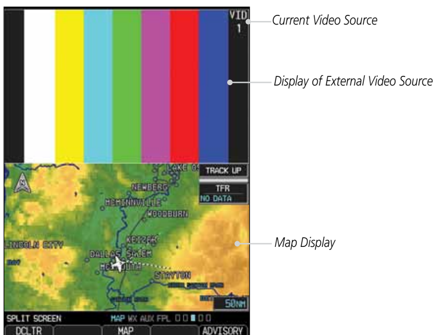
Figure 3-64 External Video
