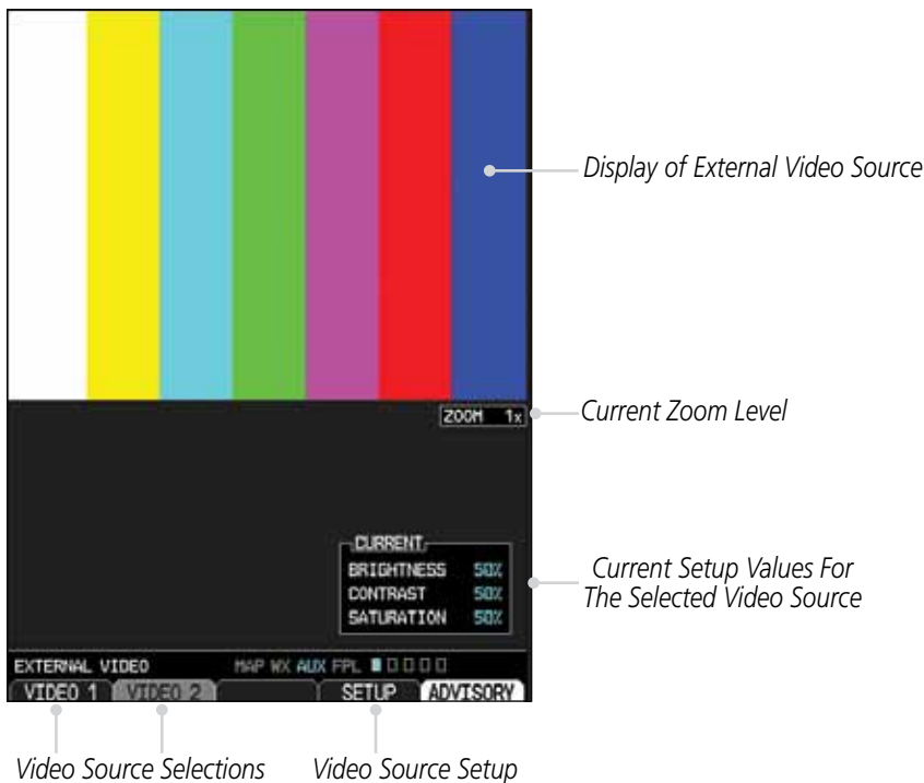
Figure 3-84 External Video
