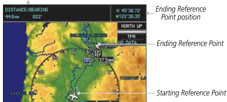
Figure 3-12 Bearing/Distance Measurement
