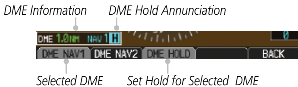
Figure 2-41 DME Indication
