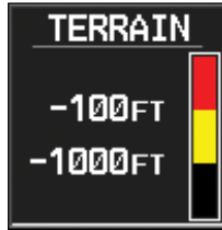
Figure 4-1 Terrain Scale
