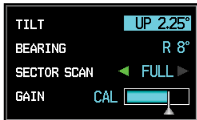
Figure 4-69 Adjusting Tilt
