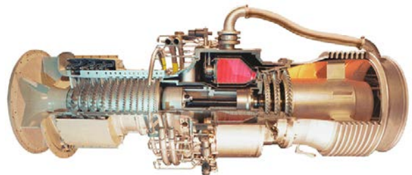
Figure 1. Gas Turbine Core Engine
