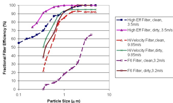
Figure 10. Comparison of Fractional Efficiency for Filter Elements from Different Suppliers and Different Face Velocities in New and Dirty Conditions (Kurz and Brun, 2012)
