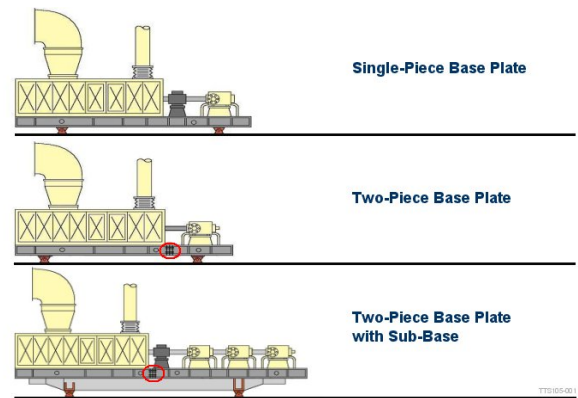
Figure 21. Base-Plate Design
