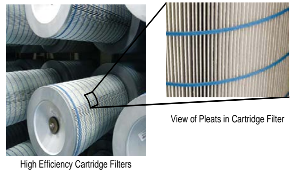
Figure 15. High Efficiency Cartridge Filters
