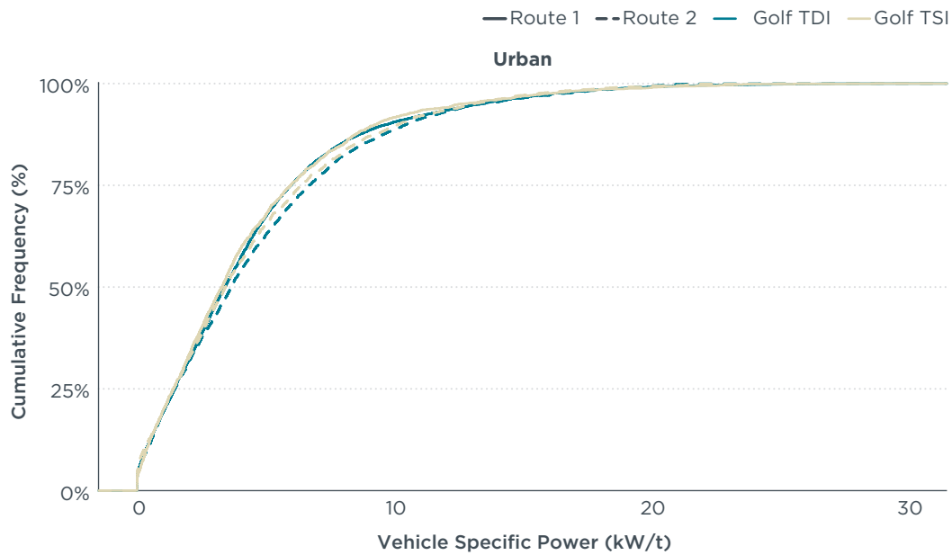
Figure 18. Comparison of the average cumulative VSP distribution for the urban speed bin. The tests performed with both vehicles on Routes 1 and 2 show a good agreement in the VSP distribution.
