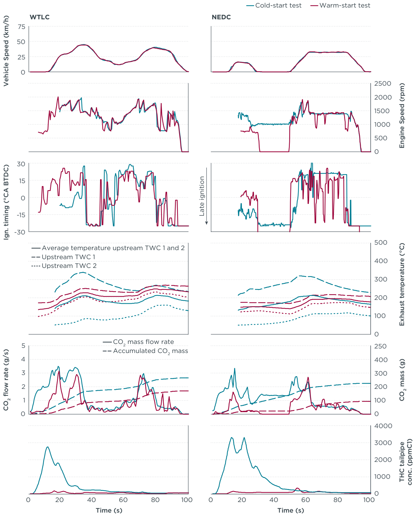
Figure 11. Golf TSI rapid catalyst heat up strategies in WLTC and NEDC at 23°C.
