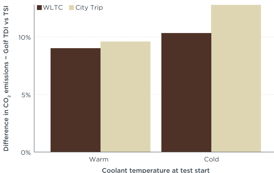
Figure 13. Comparison of the relative difference in cycle CO 2 emissions of the Golf TDI and Golf TSI for both a cold- and warm-start WLTC at 23 °C and a test with a representative duration and distance for trips performed by the German urban population.
