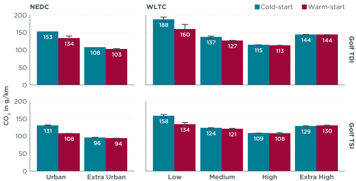
Figure 8. Comparison of phase CO 2 emission levels—Cold- versus warm-start NEDC and WLTC at 23°C. The error bar shows the minimum to maximum range of results if multiple tests were performed. No error bar is shown if only one test was performed.
