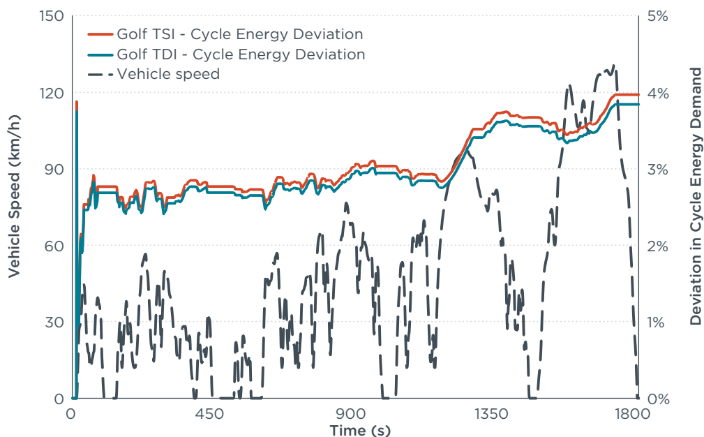
Figure 4. Relative deviation in positive cycle energy demand comparing the road load parameters used for testing with those stated by the manufacturer for comparable vehicles. The deviation is at a similar level for the Golf TDI and Golf TSI.
