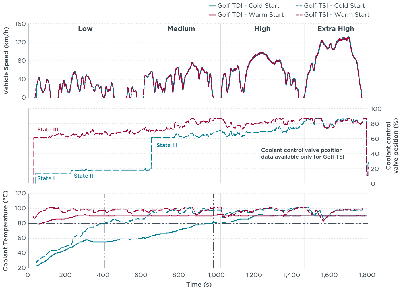
Figure 10: Coolant temperature of cold- versus warm-start WLTC at 23°C. The Golf TSI completes the engine warm-up within the low phase whereas the Golf TDI coolant temperature does not reach the warm-up threshold before the end of the medium phase. Coolant control valve data exist only for the Golf TSI. The vertical bars in the bottom graph indicate the time needed to reach 80°C coolant temperature (horizontal line) for a cold-started Golf TDI and Golf TSI test, respectively.
