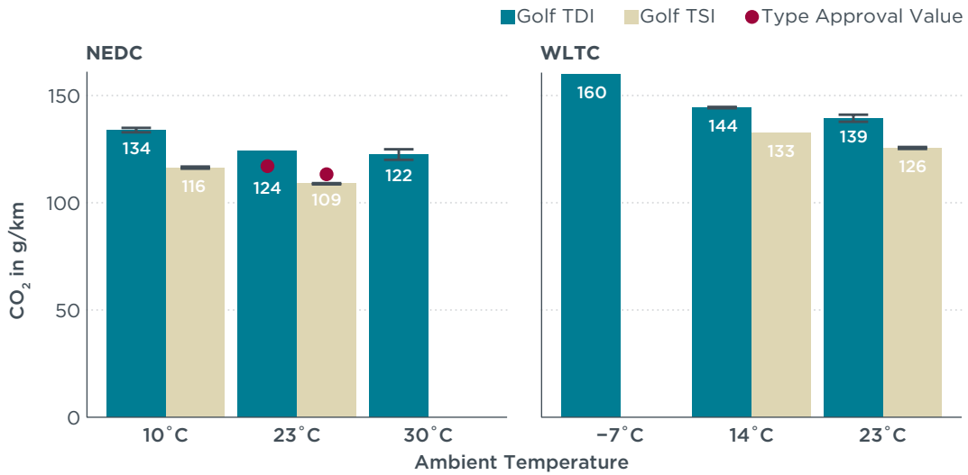
Figure 6: Effect of ambient temperature on cold-start WLTC- and NEDC-specific cycle CO 2 emissions. The error bars show the minimum to maximum range of results if multiple tests were performed. No error bar is shown if only one test was performed. The NEDC type-approval emissions are shown with red dots.
