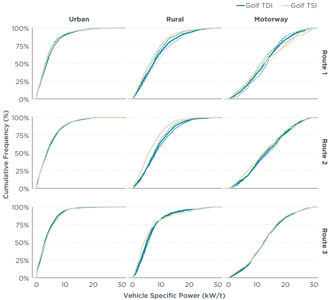
Figure 17. Cumulative distribution of VSP for the real-world driving tests performed on three different routes. In the case of multiple tests performed on one route with the same vehicle, the VSP distribution of the individual tests is shown as thin lines and the average distribution is shown in bold.
