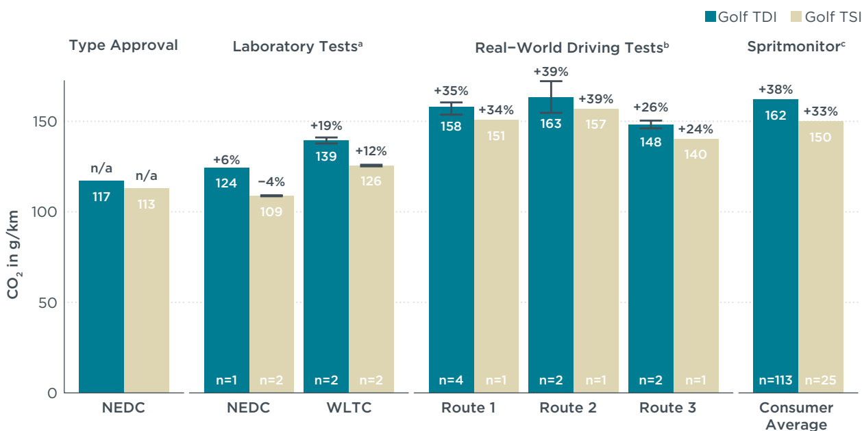
Figure ES 1. CO 2 emission levels of the Golf TDI and Golf TSI. Comparison of test results with declared type-approval values and consumer reported numbers (Spritmonitor). The error bars show the minimum to maximum range of results if multiple tests were performed. No error bar is shown if only one test was performed. The number of tests is shown at the bottom of each bar. The relationship of the CO 2 emission level to the type-approval value is shown above each bar.
