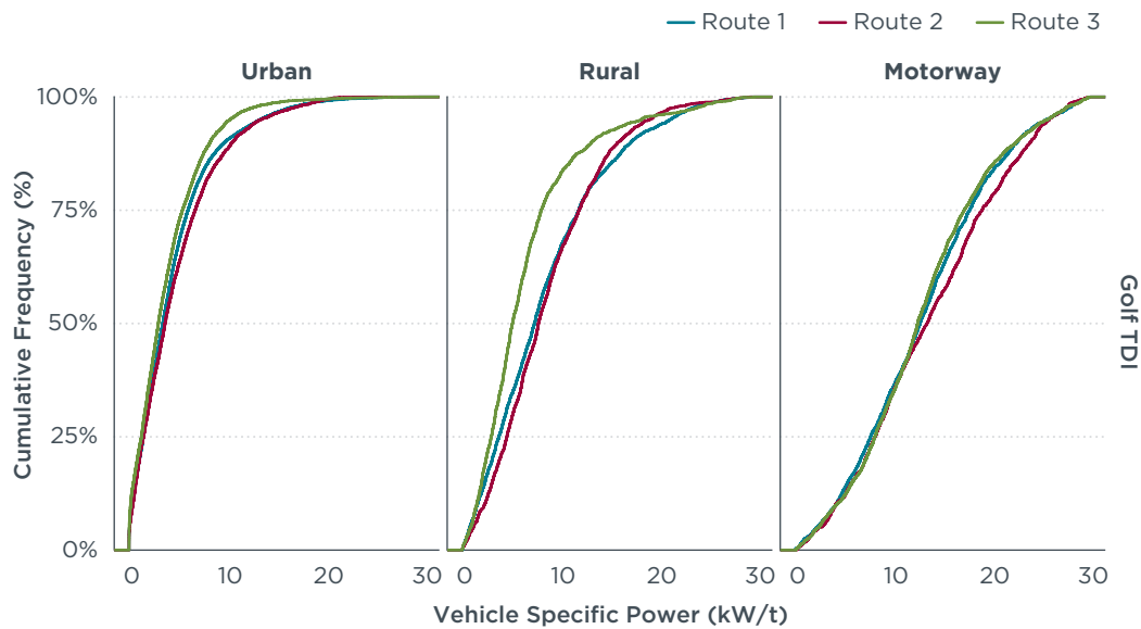
Figure 16. Comparison of the average VSP distribution of tests performed with the Golf TDI on all routes.
