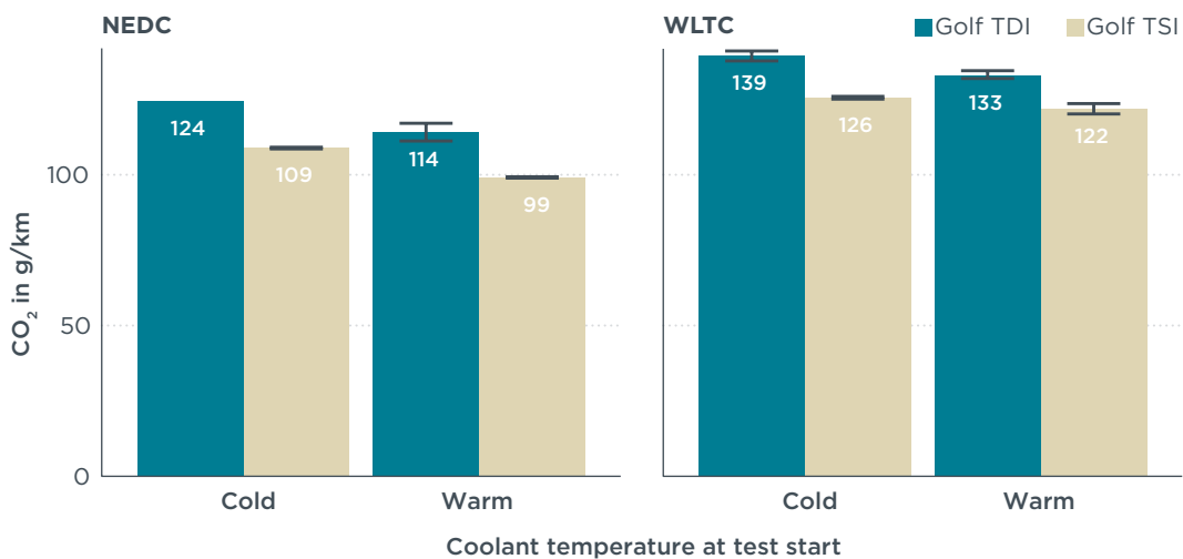
Figure 7. Effect of engine coolant temperature at test start on CO 2 emissions—Comparison of Golf TDI and Golf TSI in NEDC and WLTC tests at 23°C. The error bar shows the minimum to maximum range of results if multiple tests were performed. No error bar is shown if only one test was performed.
