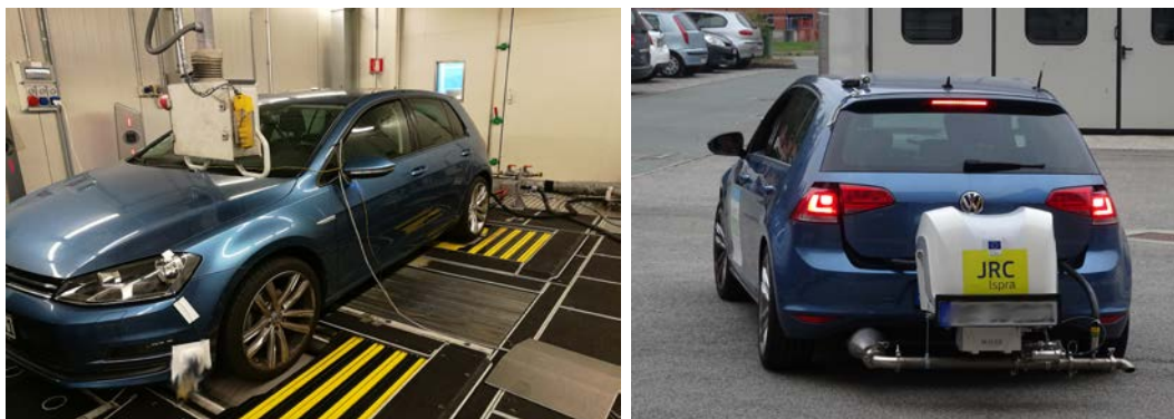
Figure 1. Golf TDI test vehicle, on chassis dynamometer and on the road with portable emissions measurement system (PEMS) installed.
