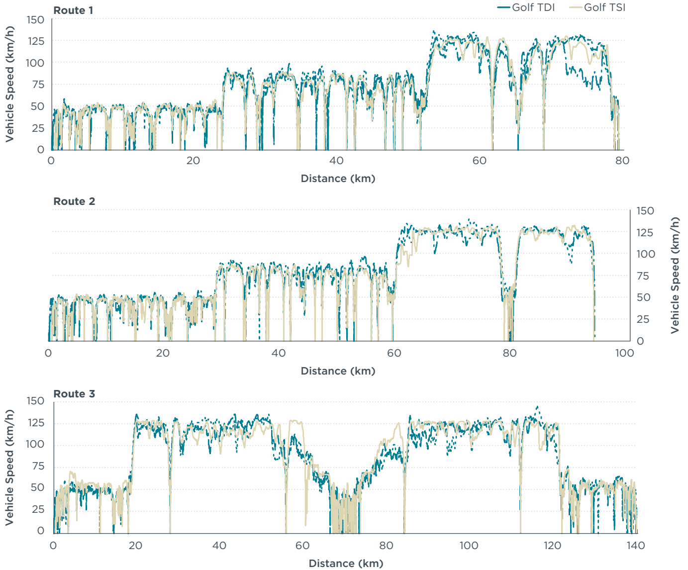
Figure 15. Speed profiles of tests performed with the Golf TDI and Golf TSI on Route 1, Route 2, and Route 3. Only one test on each route was performed with the Golf TSI. Multiple tests were performed on each route with the Golf TDI. These tests are distinguished by the line type.
