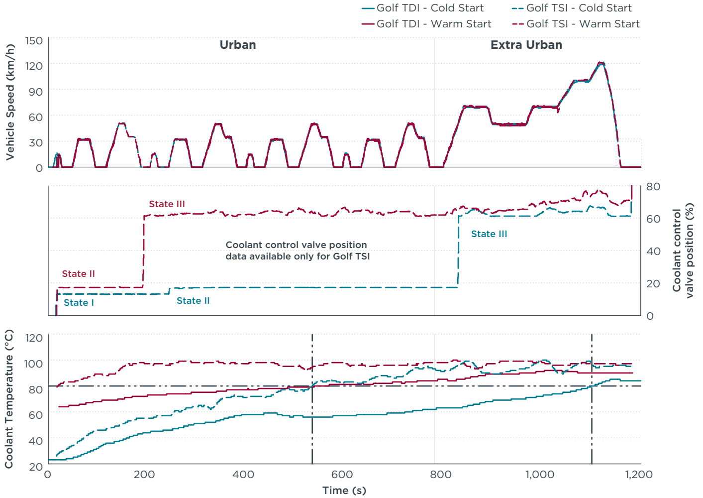
Figure 9. Coolant temperature of cold- versus warm-start NEDC at 23°C. The Golf TSI completes the engine warm-up within the urban phase whereas the Golf TDI requires approximately twice as long to reach the 80°C temperature threshold. The vertical bars in the bottom graph indicate the time needed to reach 80°C coolant temperature (horizontal line) for a cold-started Golf TDI and Golf TSI test respectively. The coolant control valve position information is available only for the Golf TSI.
