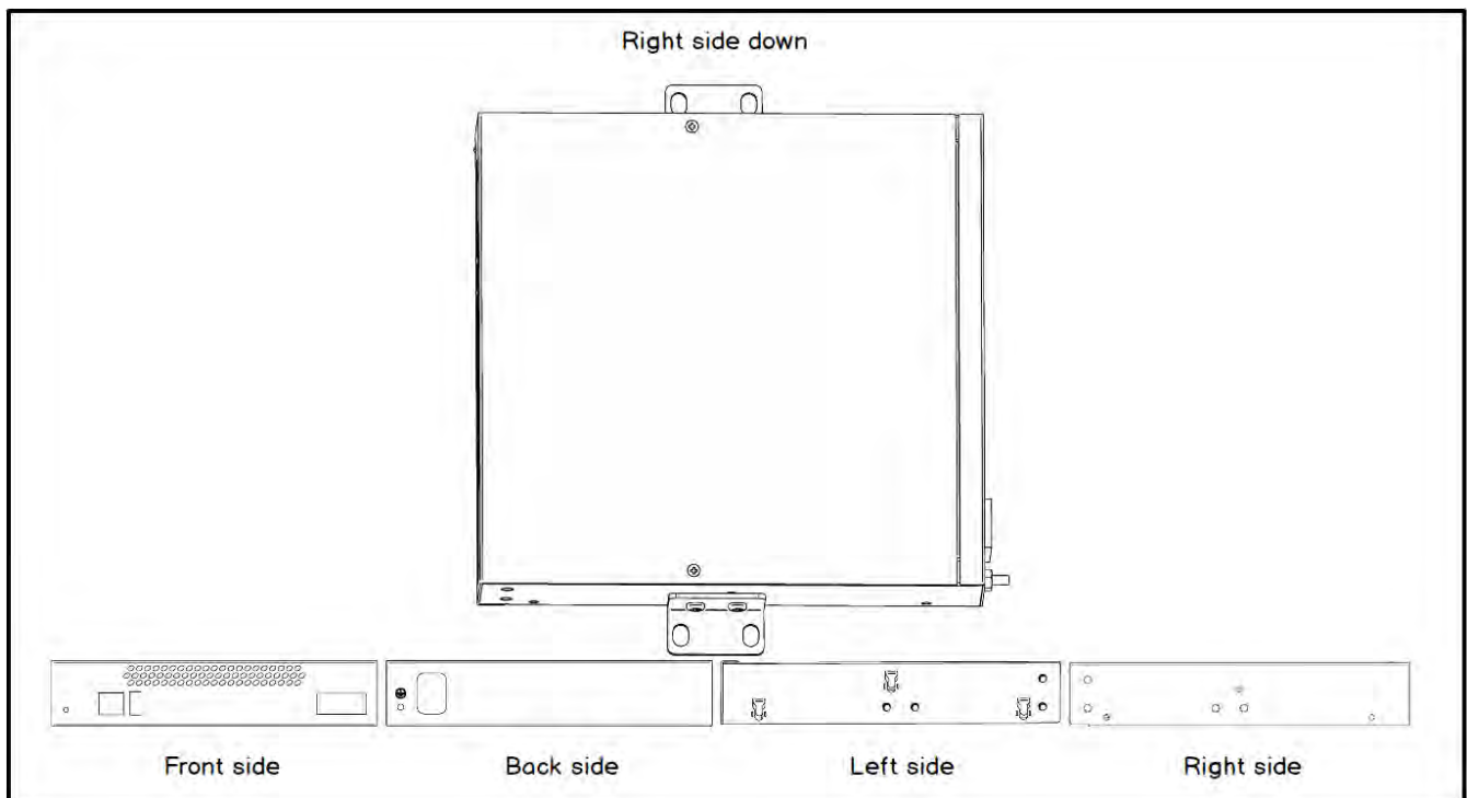
Figure 6: Acceptable Wall Mount Orientation
