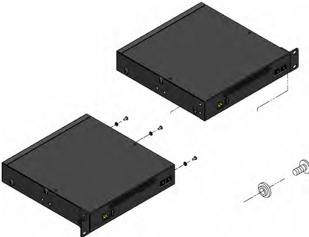
Figure 5: Side-by-side Rack Mounting
