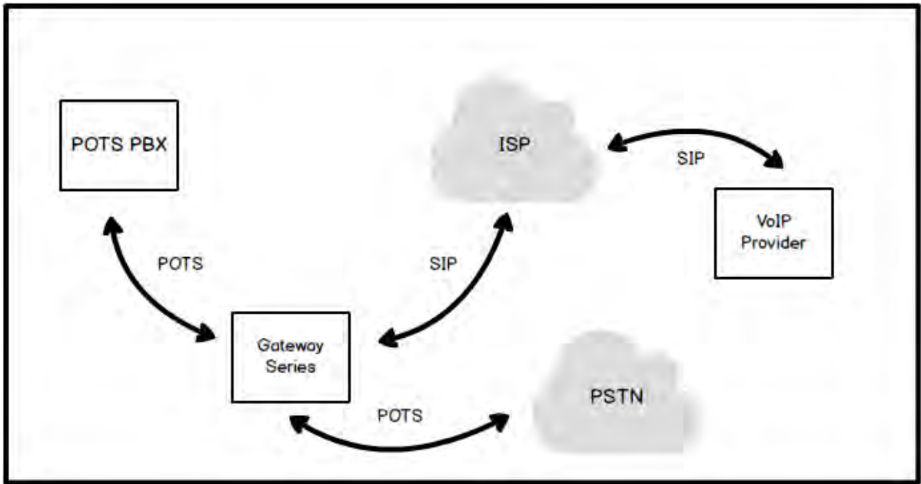
Figure 3: POTS PBX to POTS and VoIP Scenario
