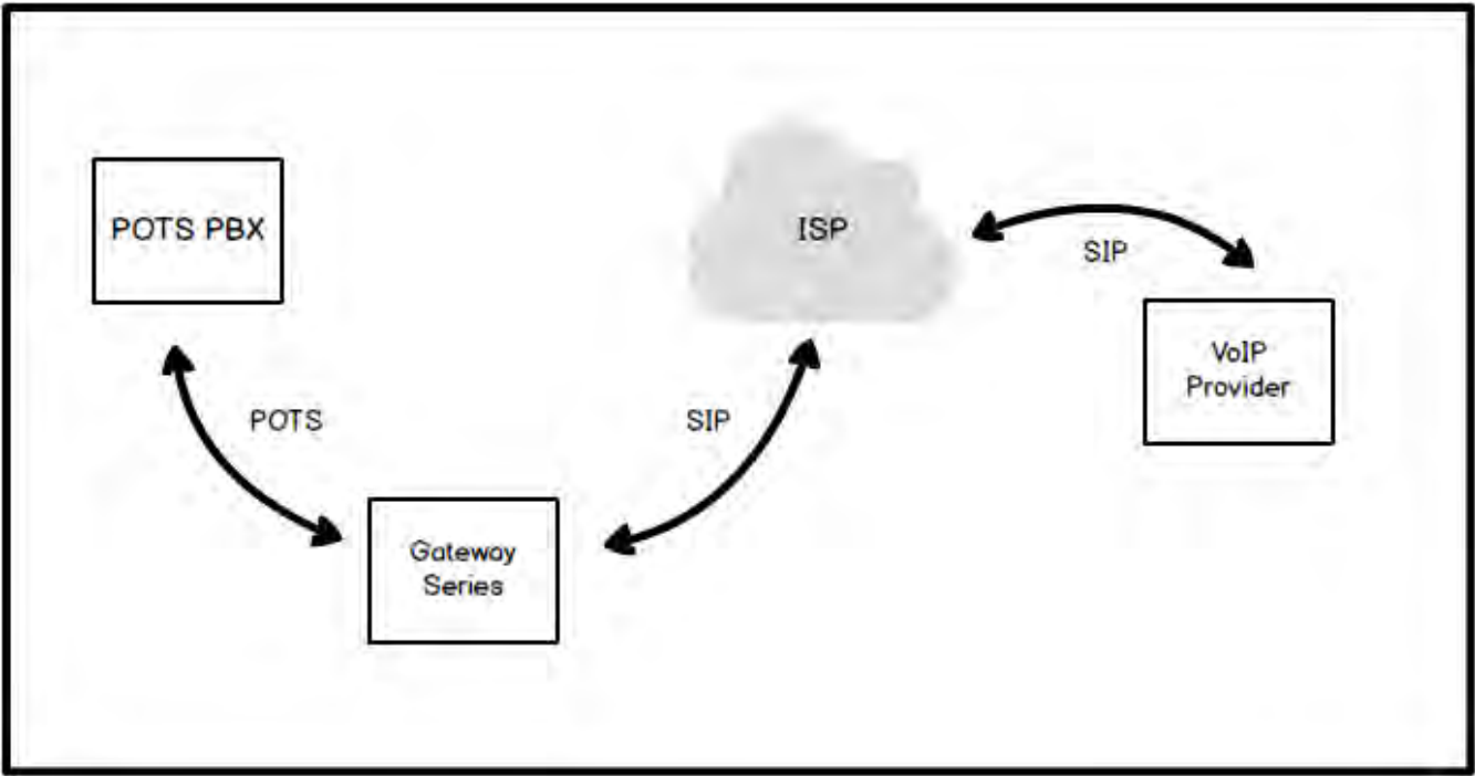
Figure 1: POTS PBX to VoIP Scenario
