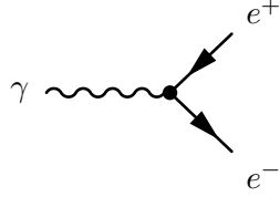
Figure 1. Feynman diagram representing the process \gamma \rightarrow e^+e^- .
