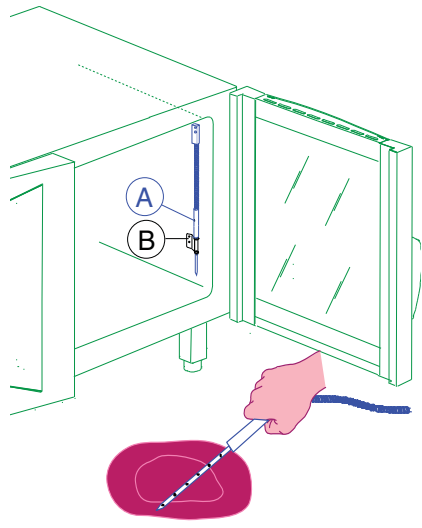
—————MULTIPOINT 6-sensor core probe
